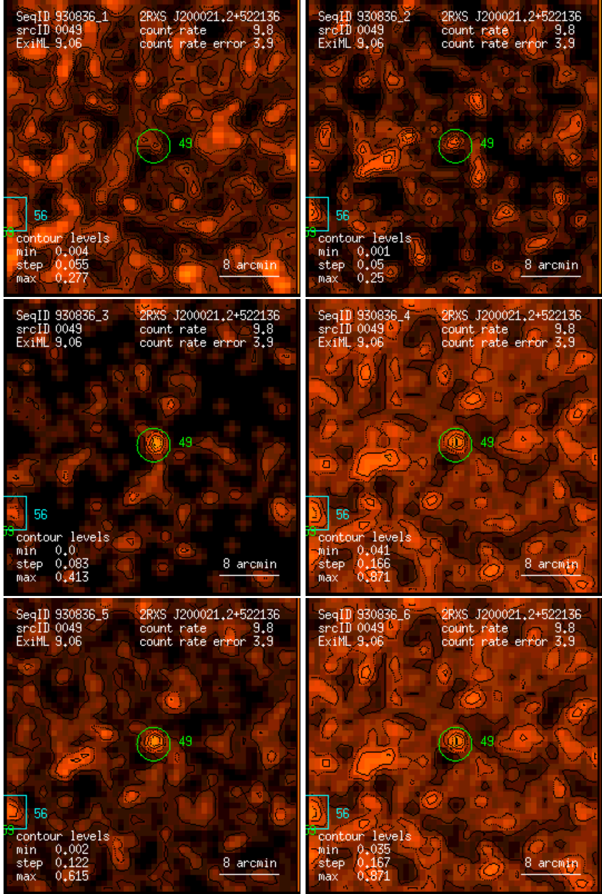
Figure 49: RASS 930836: detection 0049: band rate images, Gaussian filter: (1) PSPC channels 11 – 41, (2) 52 – 90, (3) 91 – 201, (4) 11 – 235, (5) 52 – 201, (6) 11 – 201. Broad band rates in counts/ks. Band rate contour levels in counts/ks/arcmin 2 .
