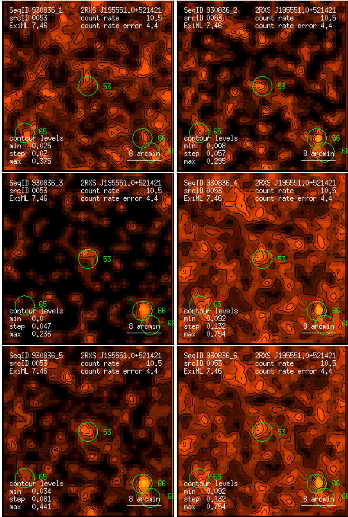
Figure 53: RASS 930836: detection 0053: band rate images, Gaussian filter: (1) PSPC channels 11 – 41, (2) 52 – 90, (3) 91 – 201, (4) 11 – 235, (5) 52 – 201, (6) 11 – 201. Broad band rates in counts/ks. Band rate contour levels in counts/ks/arcmin 2 .
