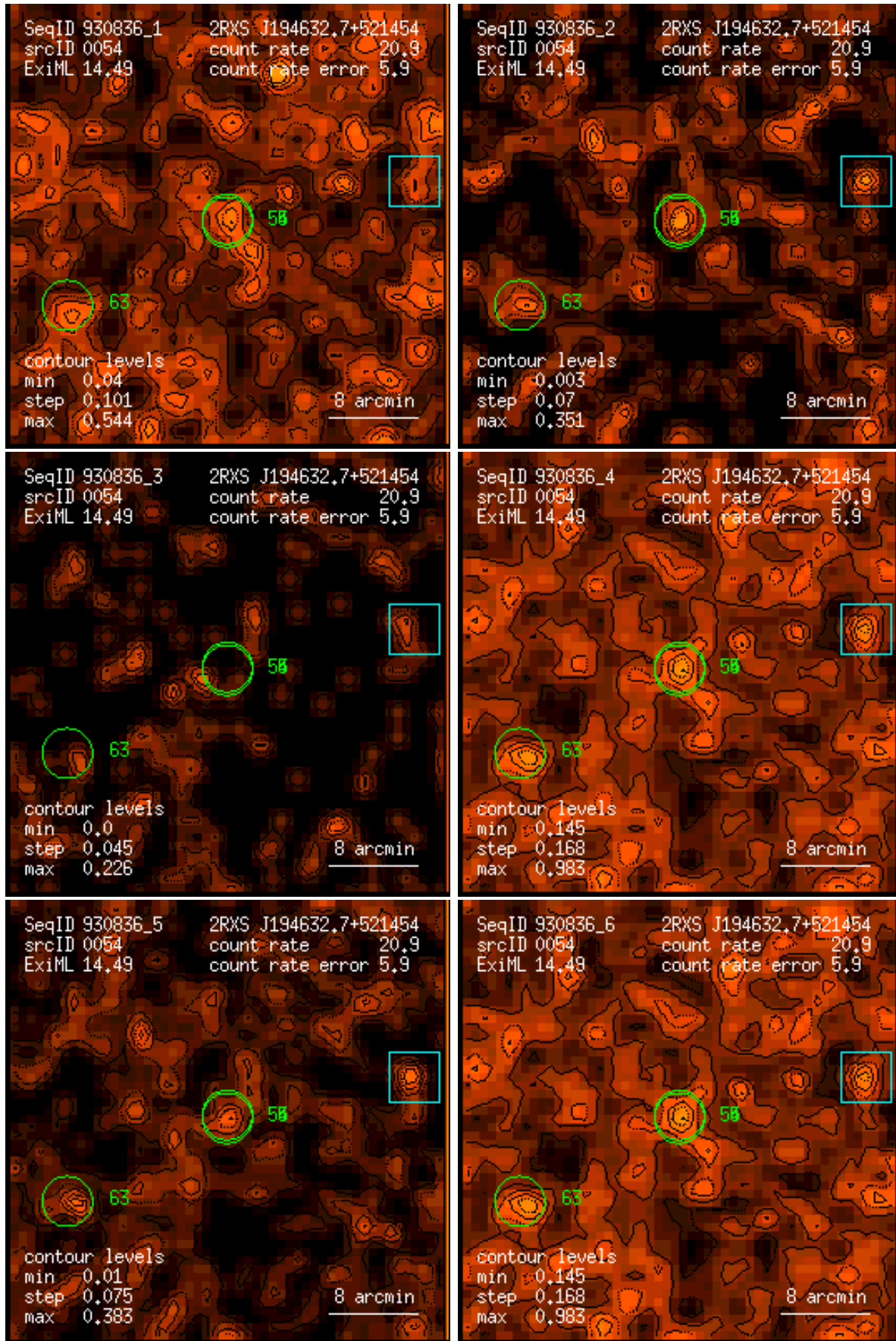
Figure 54: RASS 930836: detection 0054: band rate images, Gaussian filter: (1) PSPC channels 11 – 41, (2) 52 – 90, (3) 91 – 201, (4) 11 – 235, (5) 52 – 201, (6) 11 – 201. Broad band rates in counts/ks. Band rate contour levels in counts/ks/arcmin 2 .
