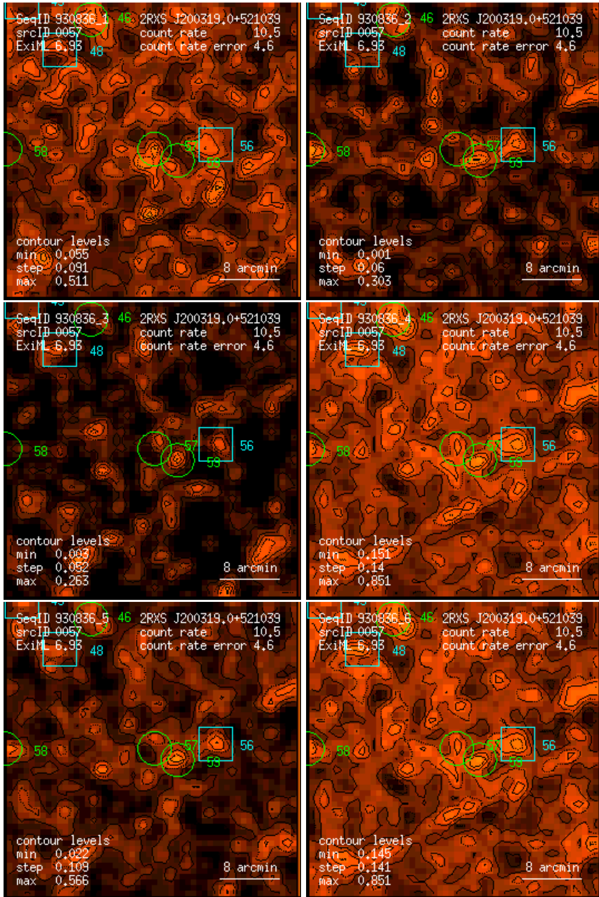
Figure 57: RASS 930836: detection 0057: band rate images, Gaussian filter: (1) PSPC channels 11 – 41, (2) 52 – 90, (3) 91 – 201, (4) 11 – 235, (5) 52 – 201, (6) 11 – 201. Broad band rates in counts/ks. Band rate contour levels in counts/ks/arcmin 2 .
