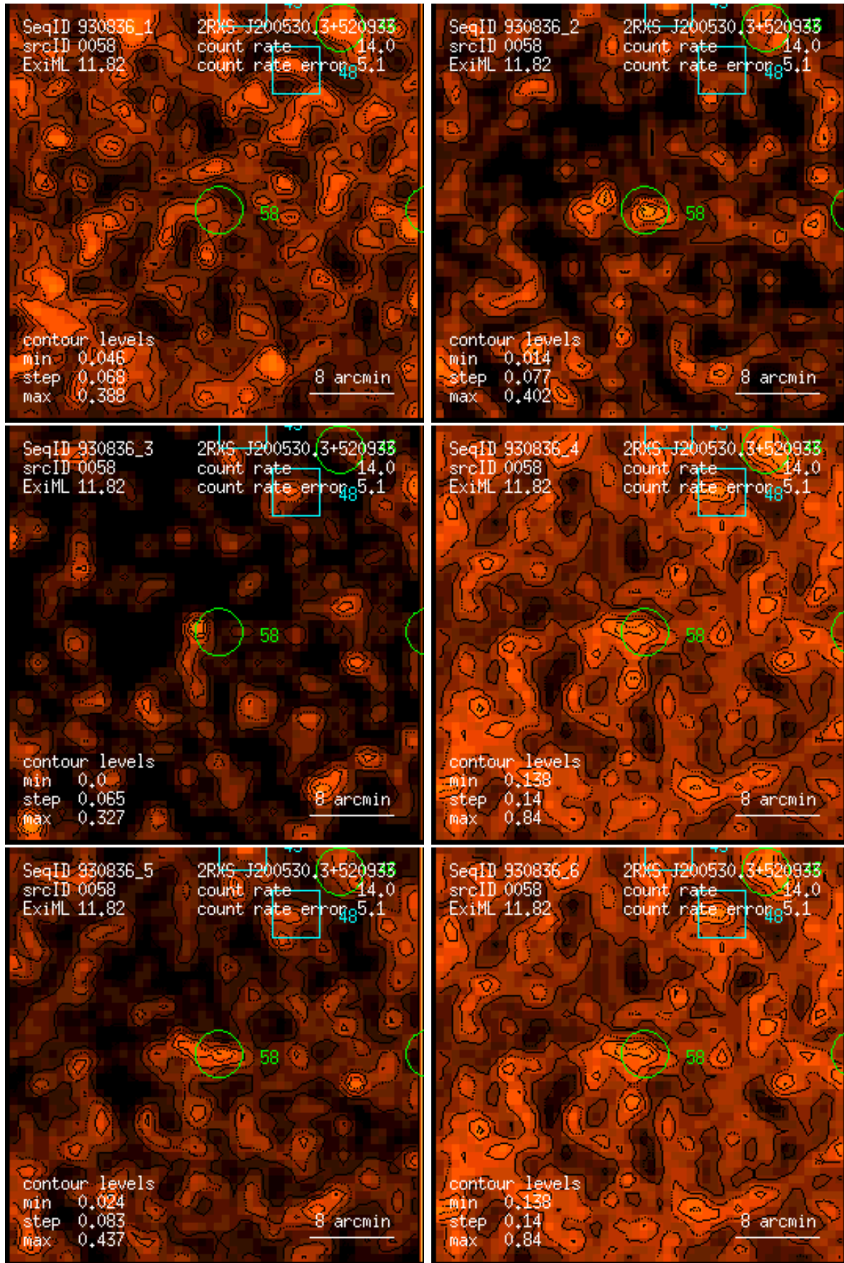
Figure 58: RASS 930836: detection 0058: band rate images, Gaussian filter: (1) PSPC channels 11 – 41, (2) 52 – 90, (3) 91 – 201, (4) 11 – 235, (5) 52 – 201, (6) 11 – 201. Broad band rates in counts/ks. Band rate contour levels in counts/ks/arcmin 2 .
