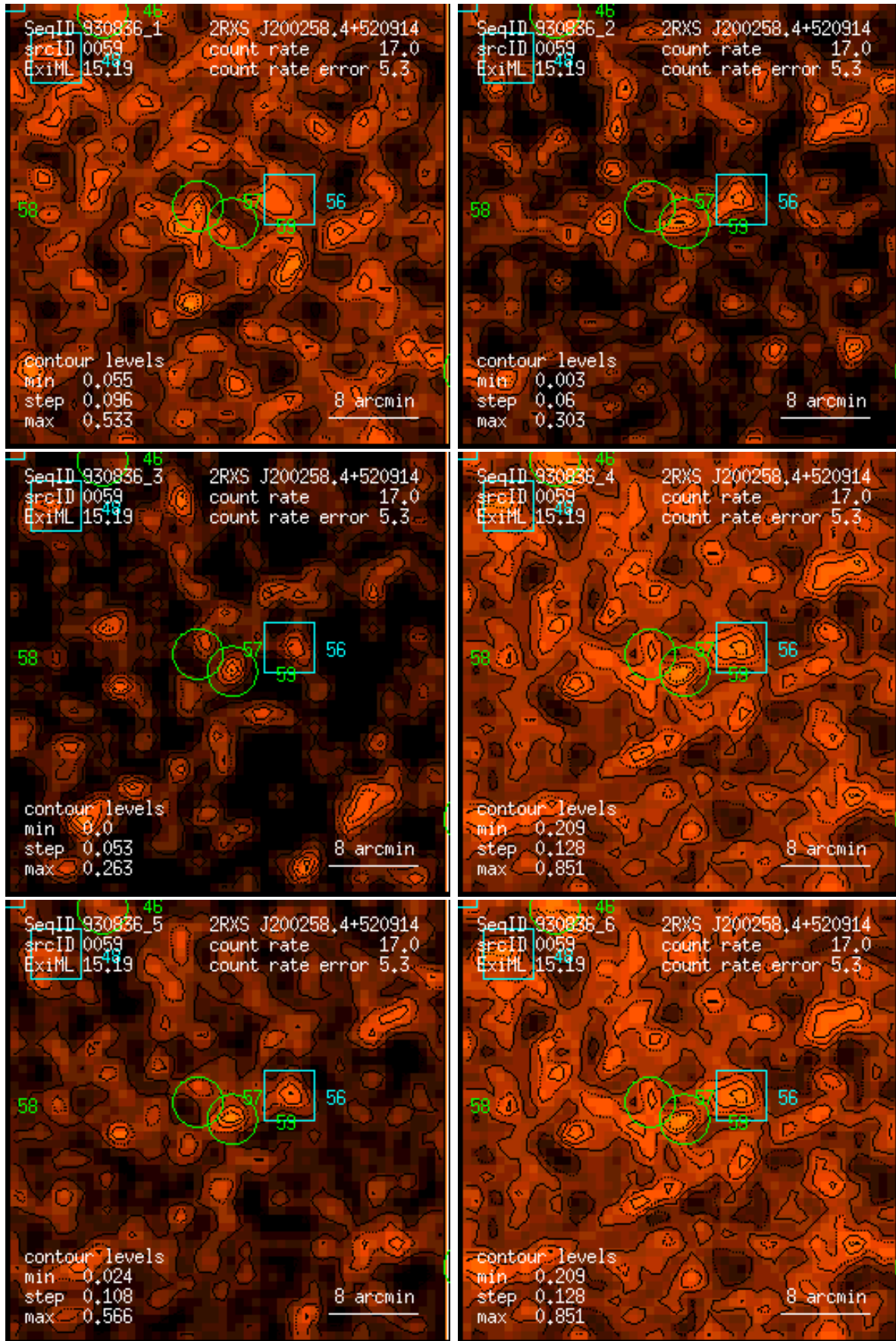
Figure 59: RASS 930836: detection 0059: band rate images, Gaussian filter: (1) PSPC channels 11 – 41, (2) 52 – 90, (3) 91 – 201, (4) 11 – 235, (5) 52 – 201, (6) 11 – 201. Broad band rates in counts/ks. Band rate contour levels in counts/ks/arcmin 2 .
