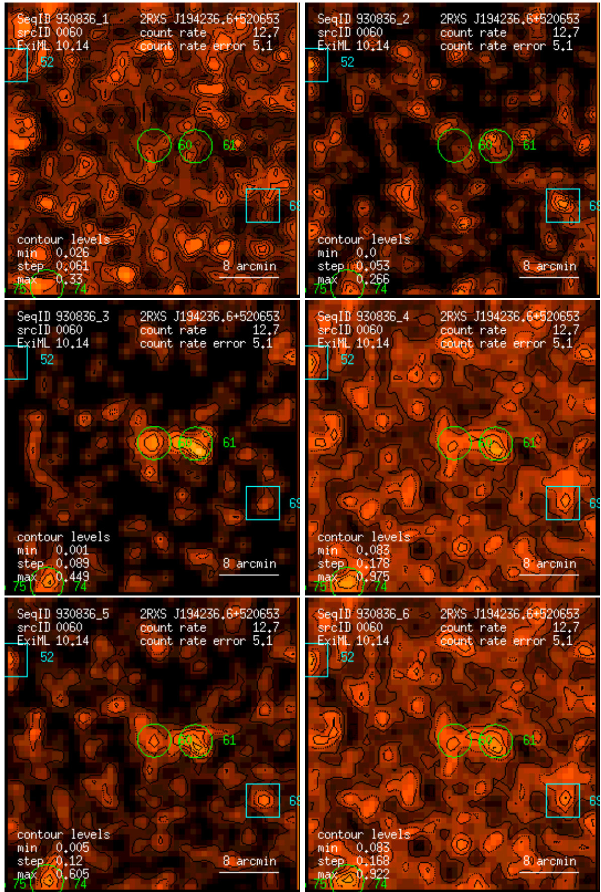
Figure 60: RASS 930836: detection 0060: band rate images, Gaussian filter: (1) PSPC channels 11 – 41, (2) 52 – 90, (3) 91 – 201, (4) 11 – 235, (5) 52 – 201, (6) 11 – 201. Broad band rates in counts/ks. Band rate contour levels in counts/ks/arcmin 2 .
