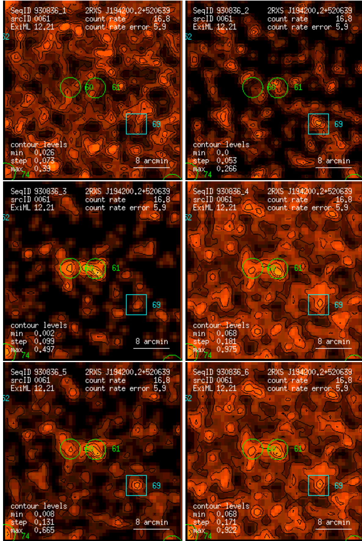
Figure 61: RASS 930836: detection 0061: band rate images, Gaussian filter: (1) PSPC channels 11 – 41, (2) 52 – 90, (3) 91 – 201, (4) 11 – 235, (5) 52 – 201, (6) 11 – 201. Broad band rates in counts/ks. Band rate contour levels in counts/ks/arcmin 2 .
