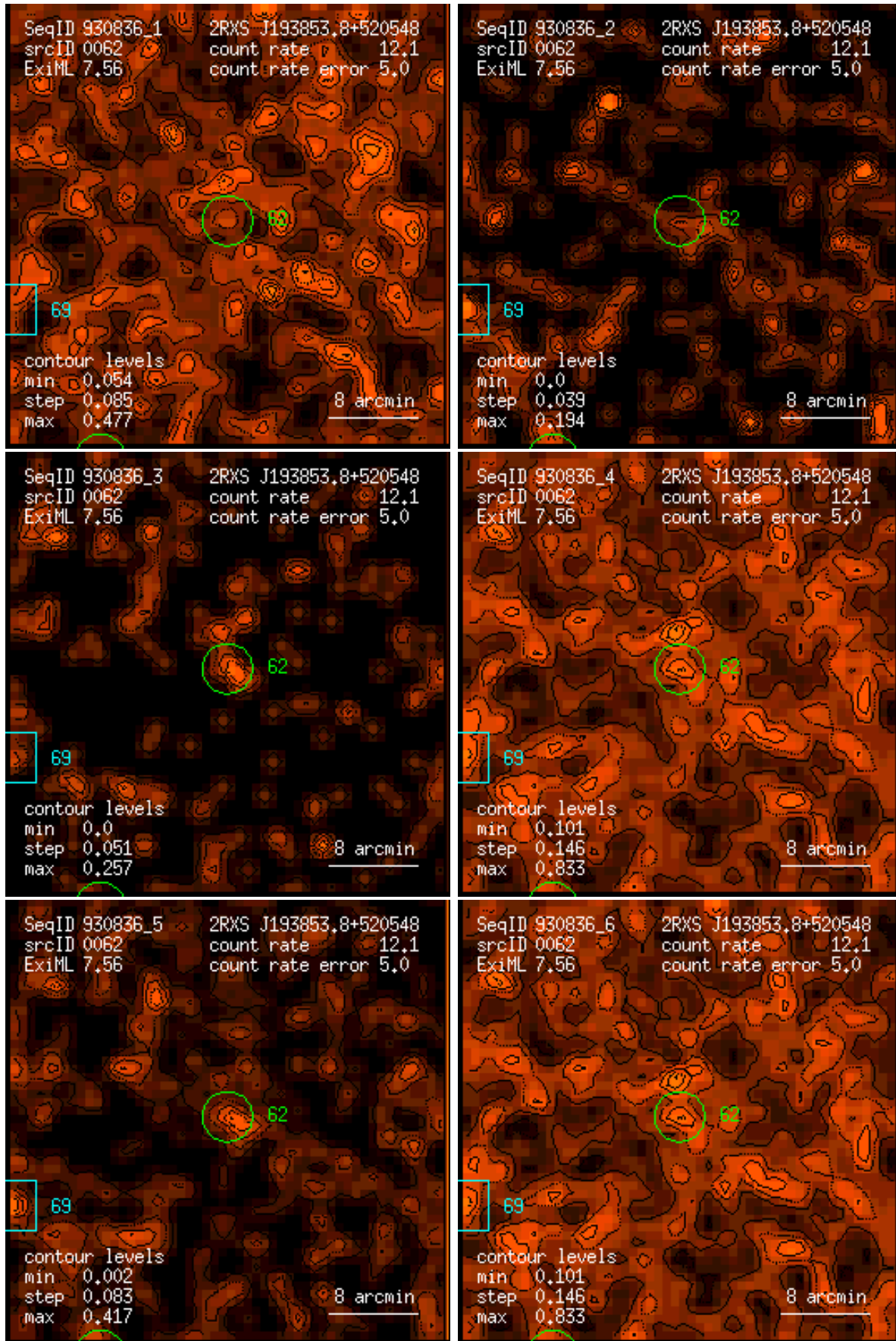
Figure 62: RASS 930836: detection 0062: band rate images, Gaussian filter: (1) PSPC channels 11 – 41, (2) 52 – 90, (3) 91 – 201, (4) 11 – 235, (5) 52 – 201, (6) 11 – 201. Broad band rates in counts/ks. Band rate contour levels in counts/ks/arcmin 2 .
