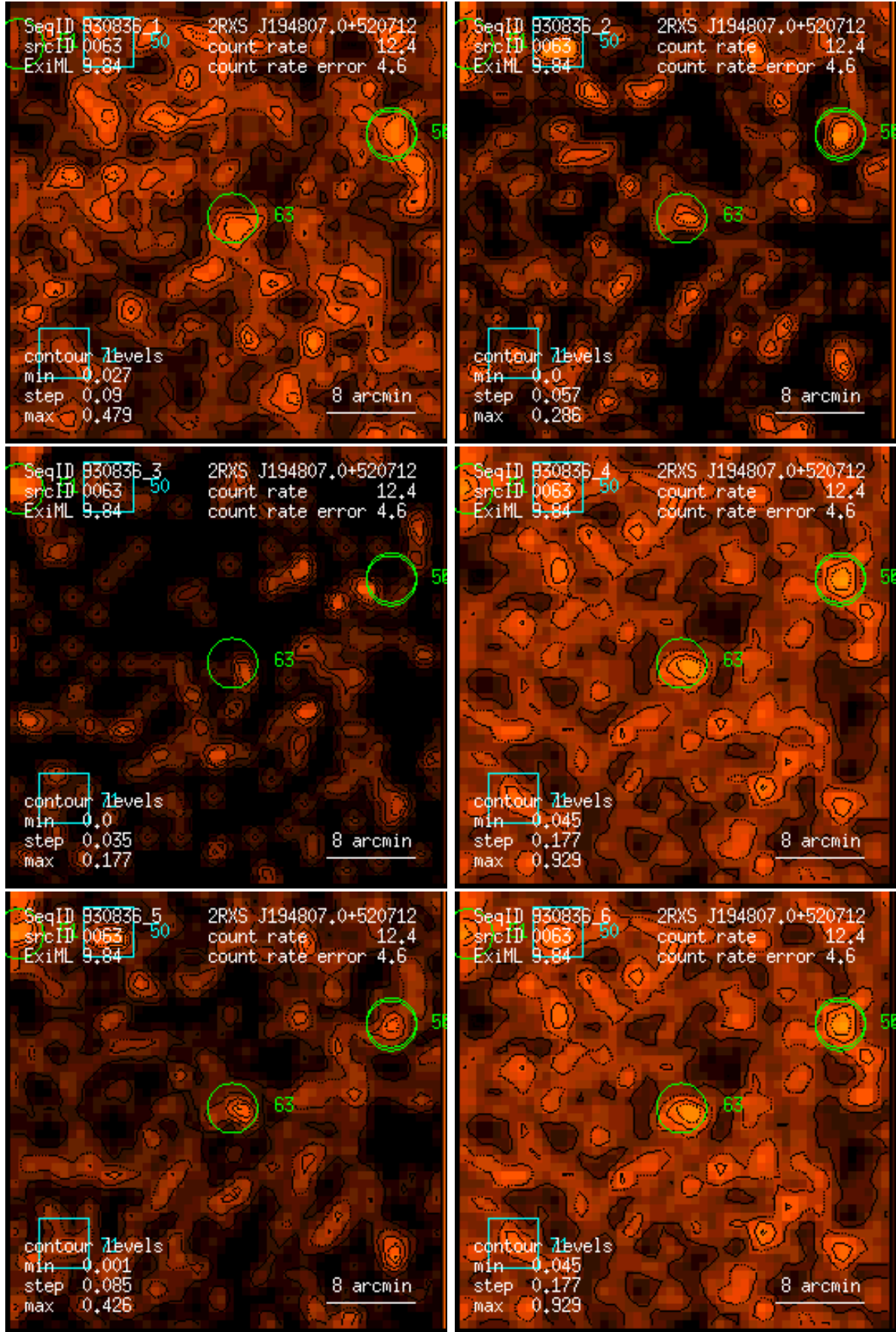
Figure 63: RASS 930836: detection 0063: band rate images, Gaussian filter: (1) PSPC channels 11 – 41, (2) 52 – 90, (3) 91 – 201, (4) 11 – 235, (5) 52 – 201, (6) 11 – 201. Broad band rates in counts/ks. Band rate contour levels in counts/ks/arcmin 2 .
