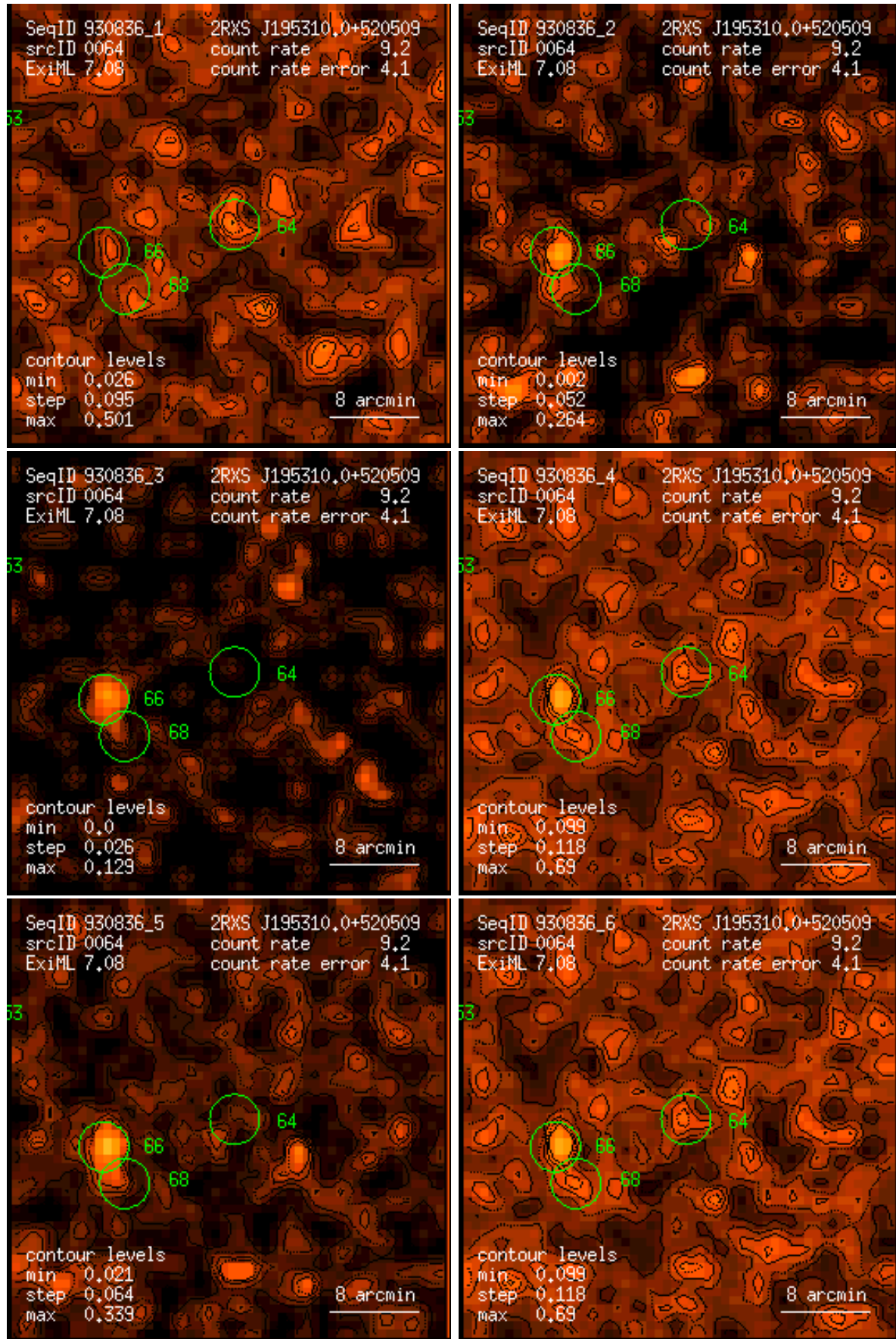
Figure 64: RASS 930836: detection 0064: band rate images, Gaussian filter: (1) PSPC channels 11 – 41, (2) 52 – 90, (3) 91 – 201, (4) 11 – 235, (5) 52 – 201, (6) 11 – 201. Broad band rates in counts/ks. Band rate contour levels in counts/ks/arcmin 2 .
