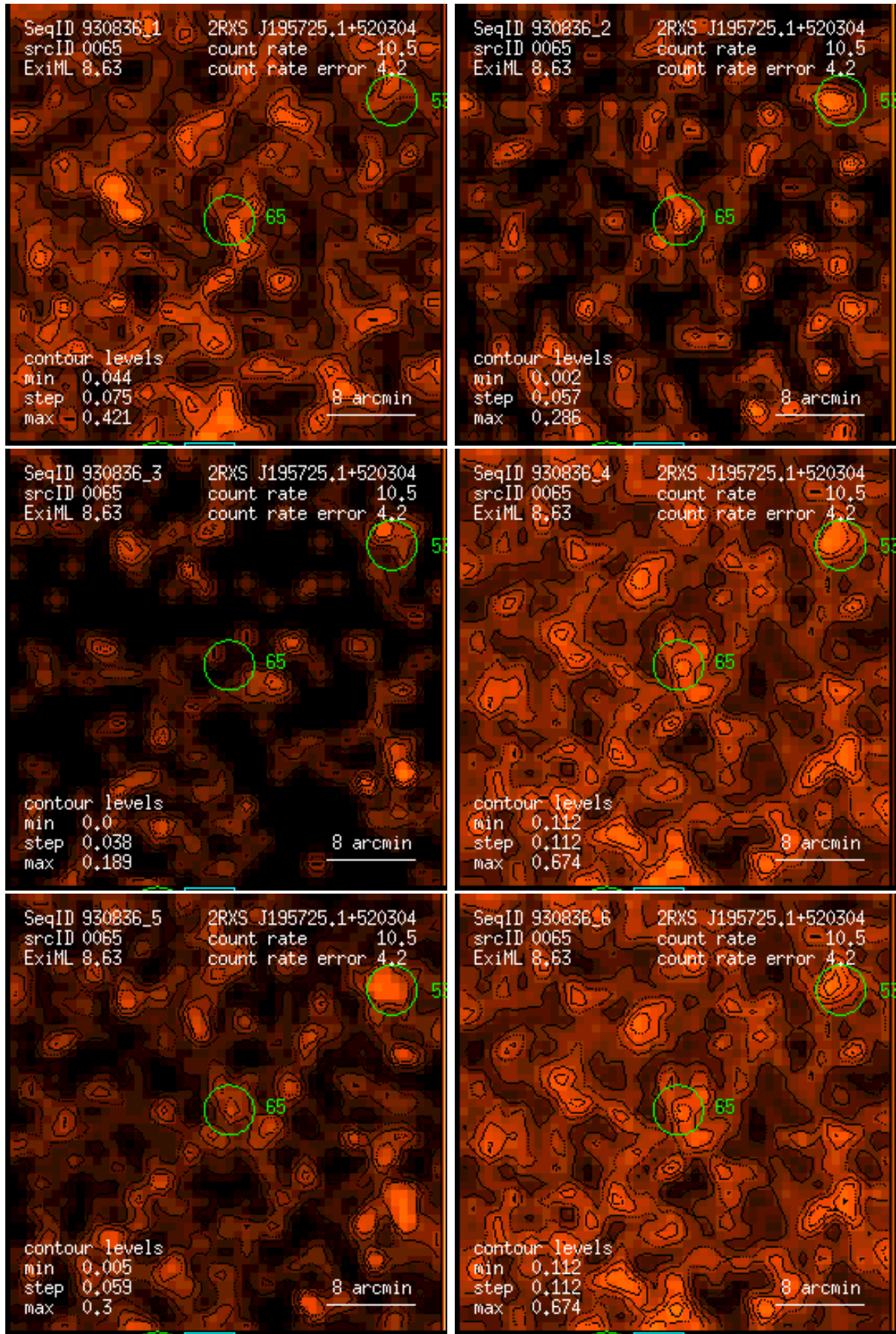
Figure 65: RASS 930836: detection 0065: band rate images, Gaussian filter: (1) PSPC channels 11 – 41, (2) 52 – 90, (3) 91 – 201, (4) 11 – 235, (5) 52 – 201, (6) 11 – 201. Broad band rates in counts/ks. Band rate contour levels in counts/ks/arcmin 2 .
