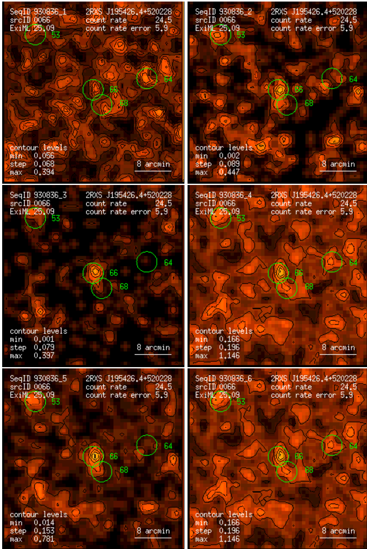
Figure 66: RASS 930836: detection 0066: band rate images, Gaussian filter: (1) PSPC channels 11 – 41, (2) 52 – 90, (3) 91 – 201, (4) 11 – 235, (5) 52 – 201, (6) 11 – 201. Broad band rates in counts/ks. Band rate contour levels in counts/ks/arcmin 2 .
