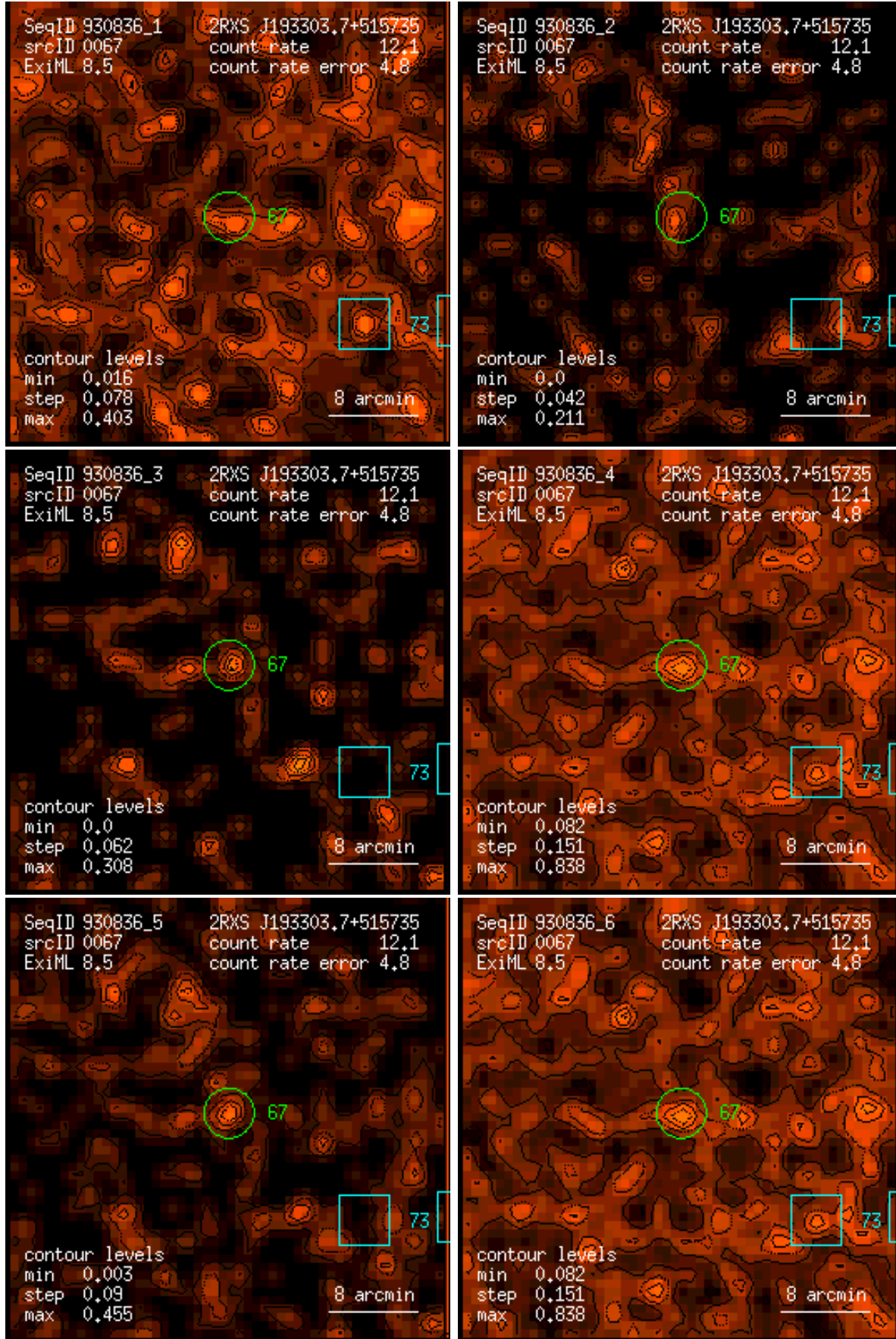
Figure 67: RASS 930836: detection 0067: band rate images, Gaussian filter: (1) PSPC channels 11 – 41, (2) 52 – 90, (3) 91 – 201, (4) 11 – 235, (5) 52 – 201, (6) 11 – 201. Broad band rates in counts/ks. Band rate contour levels in counts/ks/arcmin 2 .
