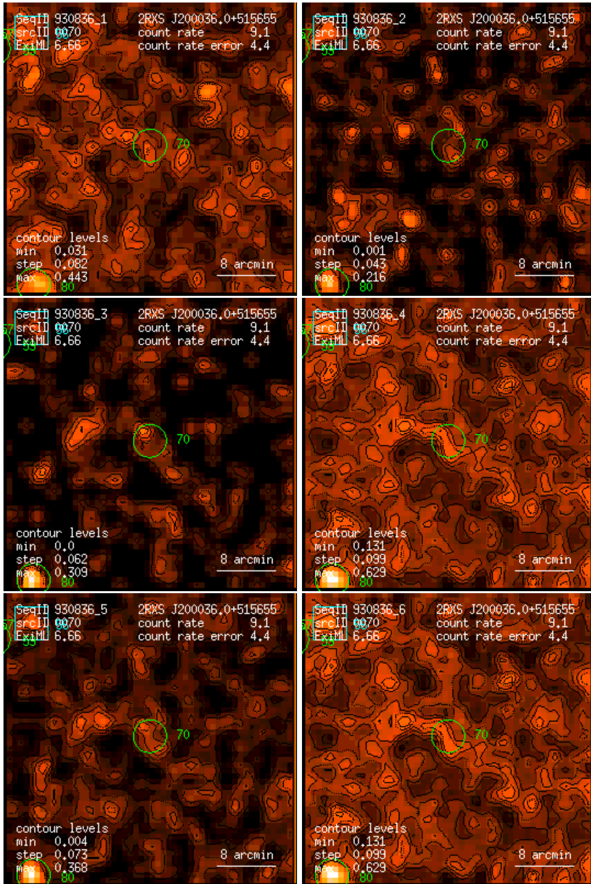
Figure 70: RASS 930836: detection 0070: band rate images, Gaussian filter: (1) PSPC channels 11 – 41, (2) 52 – 90, (3) 91 – 201, (4) 11 – 235, (5) 52 – 201, (6) 11 – 201. Broad band rates in counts/ks. Band rate contour levels in counts/ks/arcmin 2 .
