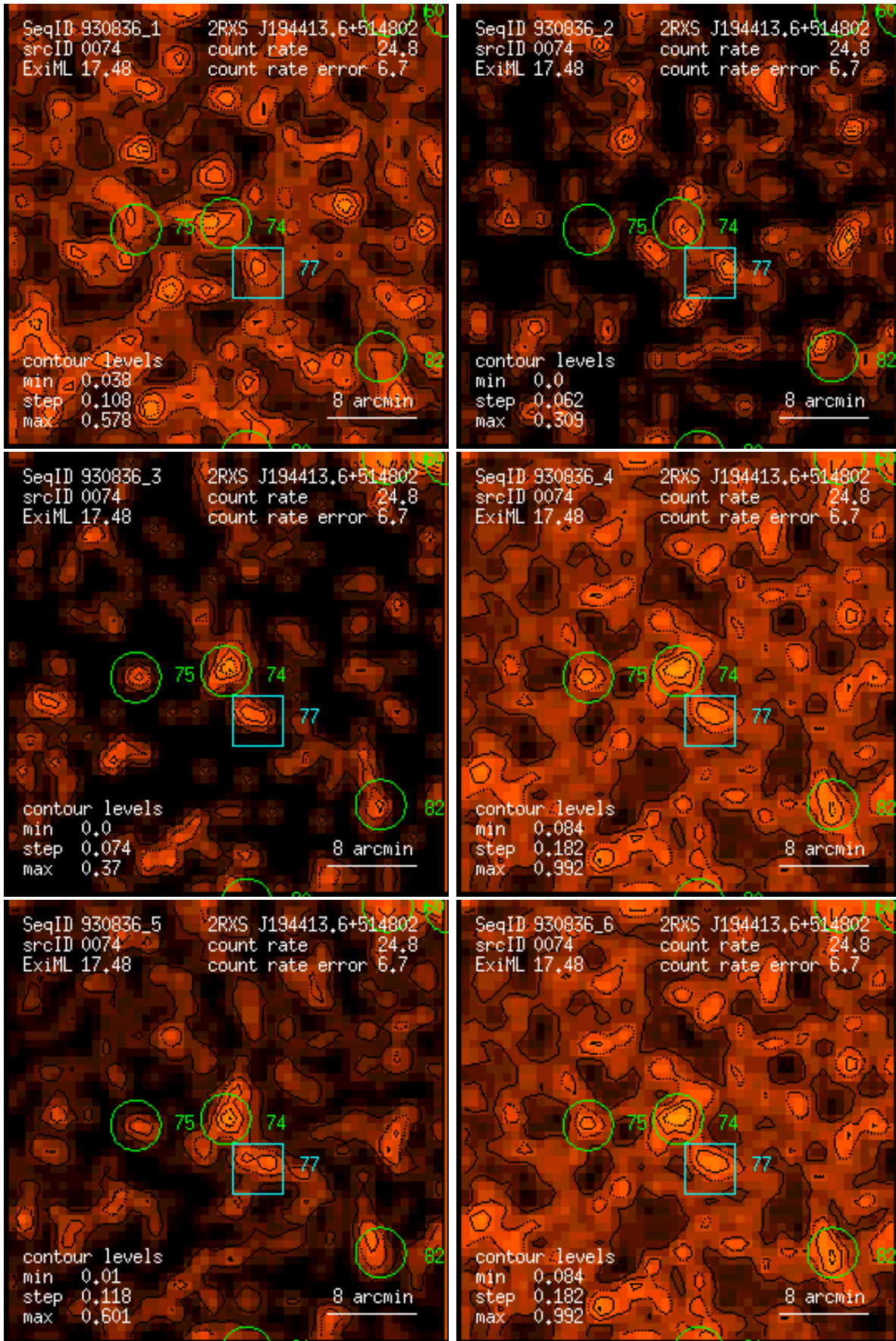
Figure 74: RASS 930836: detection 0074: band rate images, Gaussian filter: (1) PSPC channels 11 – 41, (2) 52 – 90, (3) 91 – 201, (4) 11 – 235, (5) 52 – 201, (6) 11 – 201. Broad band rates in counts/ks. Band rate contour levels in counts/ks/arcmin 2 .
