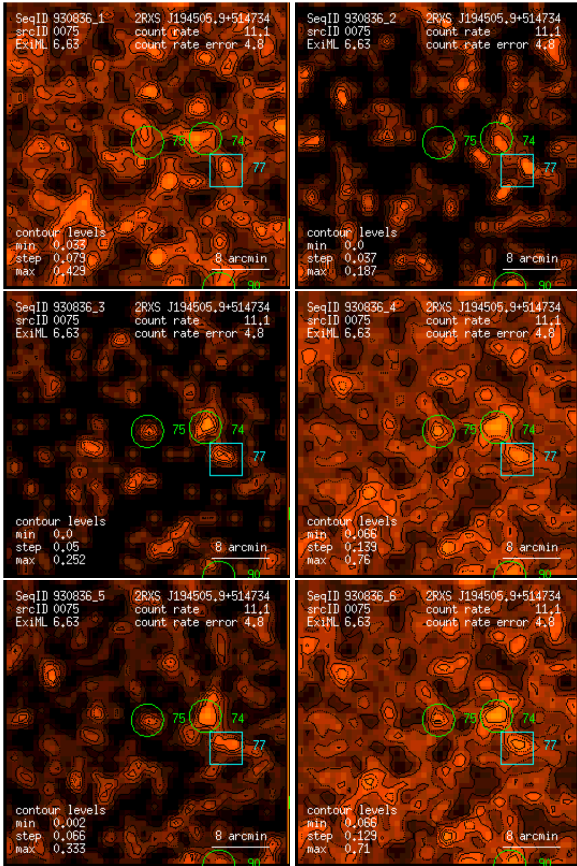
Figure 75: RASS 930836: detection 0075: band rate images, Gaussian filter: (1) PSPC channels 11 – 41, (2) 52 – 90, (3) 91 – 201, (4) 11 – 235, (5) 52 – 201, (6) 11 – 201. Broad band rates in counts/ks. Band rate contour levels in counts/ks/arcmin 2 .
