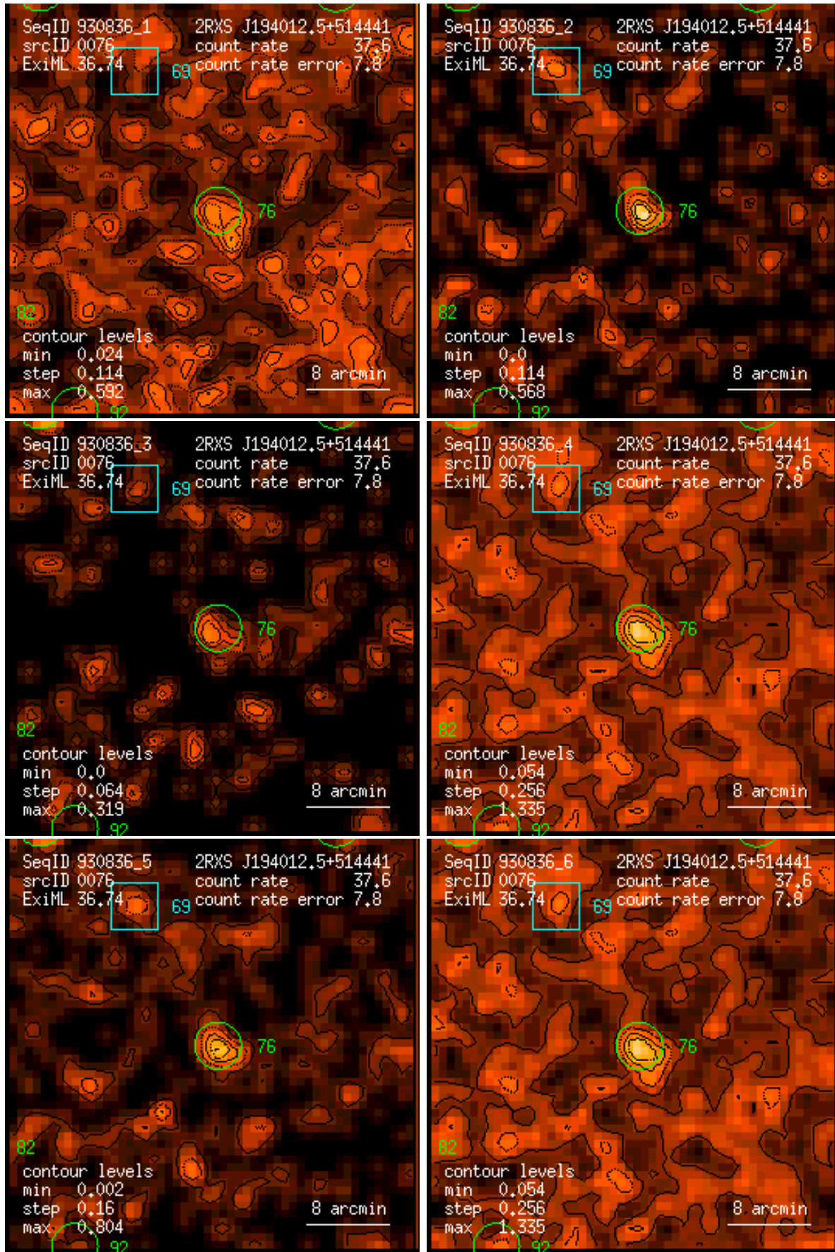
Figure 76: RASS 930836: detection 0076: band rate images, Gaussian filter: (1) PSPC channels 11 – 41, (2) 52 – 90, (3) 91 – 201, (4) 11 – 235, (5) 52 – 201, (6) 11 – 201. Broad band rates in counts/ks. Band rate contour levels in counts/ks/arcmin 2 .
