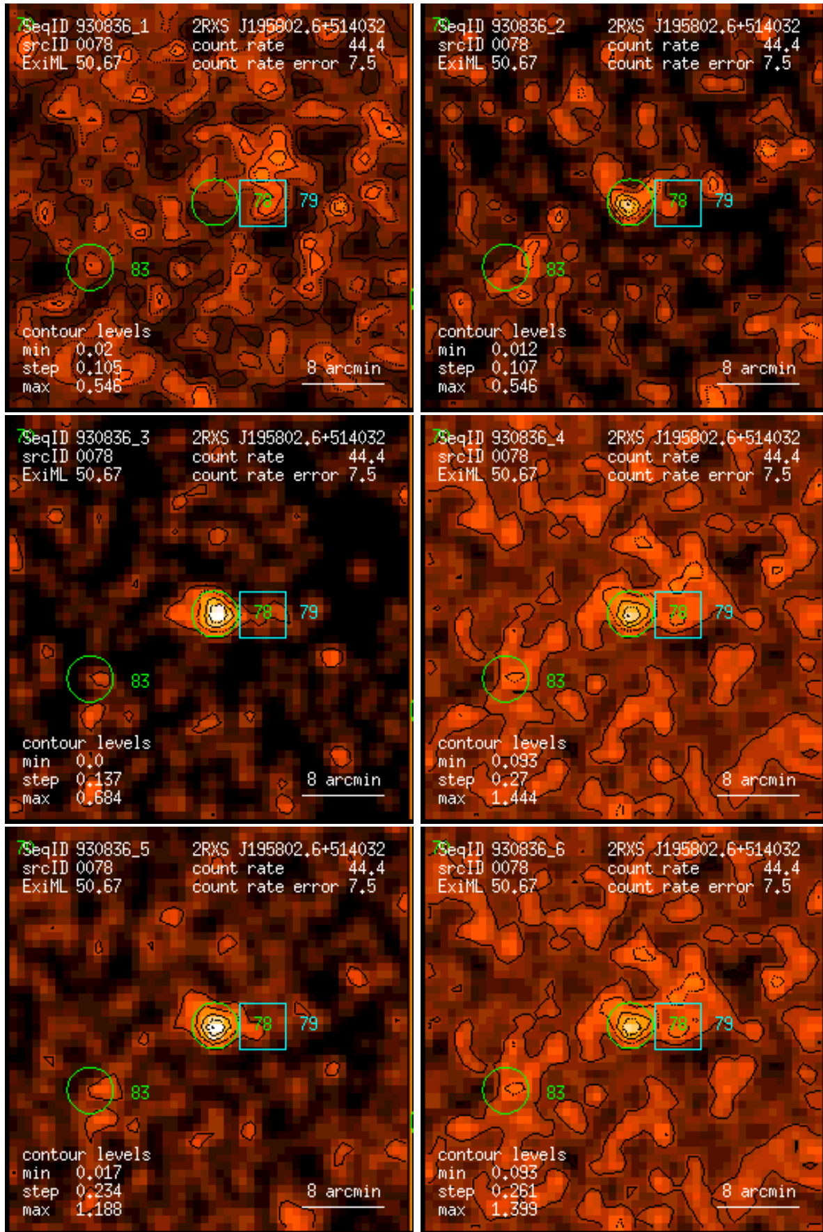
Figure 78: RASS 930836: detection 0078: band rate images, Gaussian filter: (1) PSPC channels 11 – 41, (2) 52 – 90, (3) 91 – 201, (4) 11 – 235, (5) 52 – 201, (6) 11 – 201. Broad band rates in counts/ks. Band rate contour levels in counts/ks/arcmin 2 .
