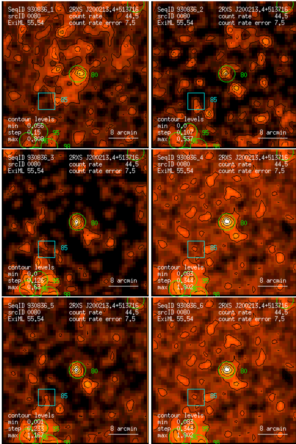
Figure 80: RASS 930836: detection 0080: band rate images, Gaussian filter: (1) PSPC channels 11 – 41, (2) 52 – 90, (3) 91 – 201, (4) 11 – 235, (5) 52 – 201, (6) 11 – 201. Broad band rates in counts/ks. Band rate contour levels in counts/ks/arcmin 2 .
