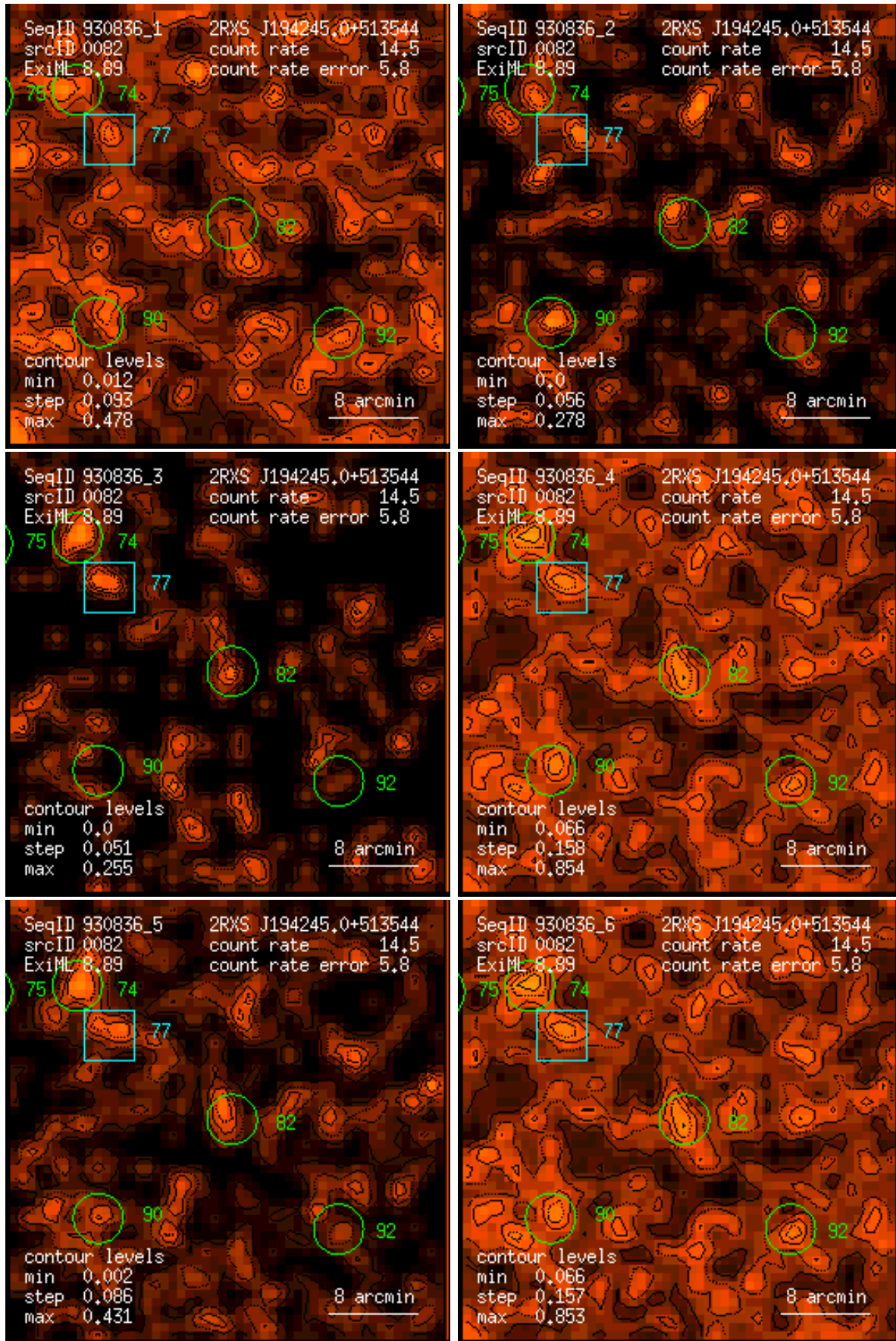
Figure 82: RASS 930836: detection 0082: band rate images, Gaussian filter: (1) PSPC channels 11 – 41, (2) 52 – 90, (3) 91 – 201, (4) 11 – 235, (5) 52 – 201, (6) 11 – 201. Broad band rates in counts/ks. Band rate contour levels in counts/ks/arcmin 2 .
