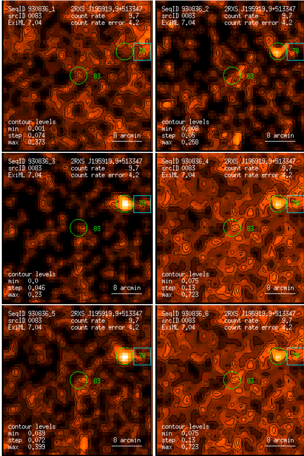
Figure 83: RASS 930836: detection 0083: band rate images, Gaussian filter: (1) PSPC channels 11 – 41, (2) 52 – 90, (3) 91 – 201, (4) 11 – 235, (5) 52 – 201, (6) 11 – 201. Broad band rates in counts/ks. Band rate contour levels in counts/ks/arcmin 2 .
