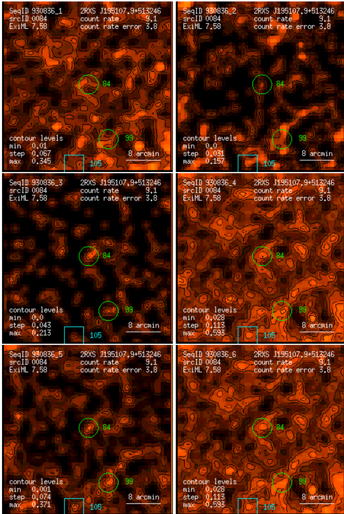
Figure 84: RASS 930836: detection 0084: band rate images, Gaussian filter: (1) PSPC channels 11 – 41, (2) 52 – 90, (3) 91 – 201, (4) 11 – 235, (5) 52 – 201, (6) 11 – 201. Broad band rates in counts/ks. Band rate contour levels in counts/ks/arcmin 2 .
