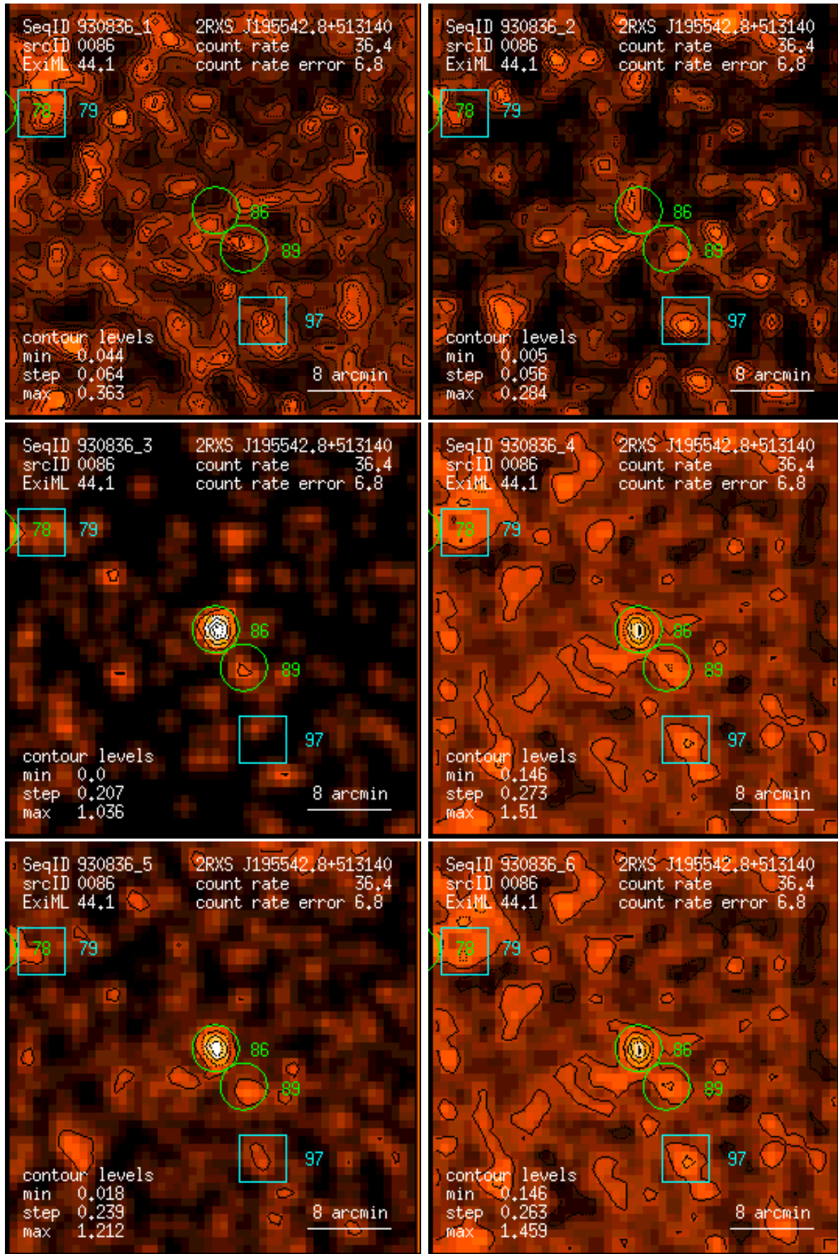
Figure 86: RASS 930836: detection 0086: band rate images, Gaussian filter: (1) PSPC channels 11 – 41, (2) 52 – 90, (3) 91 – 201, (4) 11 – 235, (5) 52 – 201, (6) 11 – 201. Broad band rates in counts/ks. Band rate contour levels in counts/ks/arcmin 2 .
