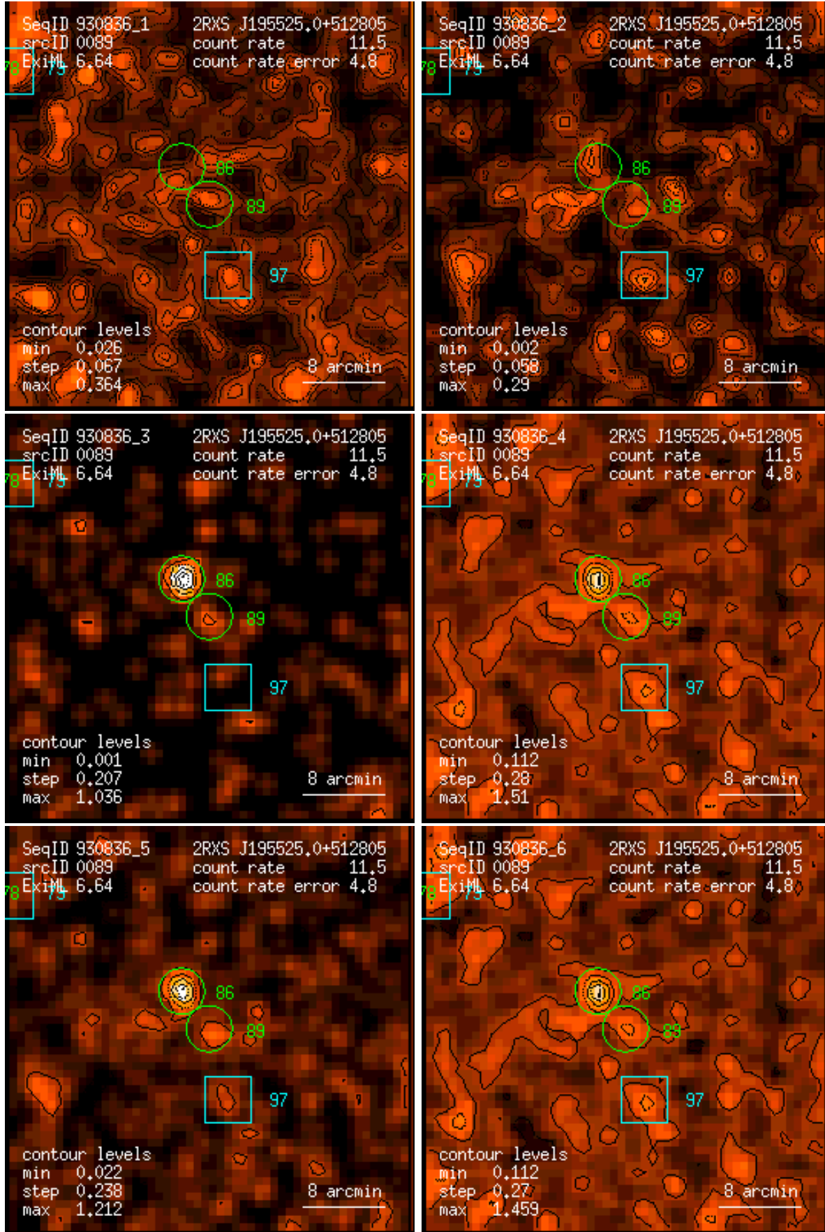
Figure 89: RASS 930836: detection 0089: band rate images, Gaussian filter: (1) PSPC channels 11 – 41, (2) 52 – 90, (3) 91 – 201, (4) 11 – 235, (5) 52 – 201, (6) 11 – 201. Broad band rates in counts/ks. Band rate contour levels in counts/ks/arcmin 2 .
