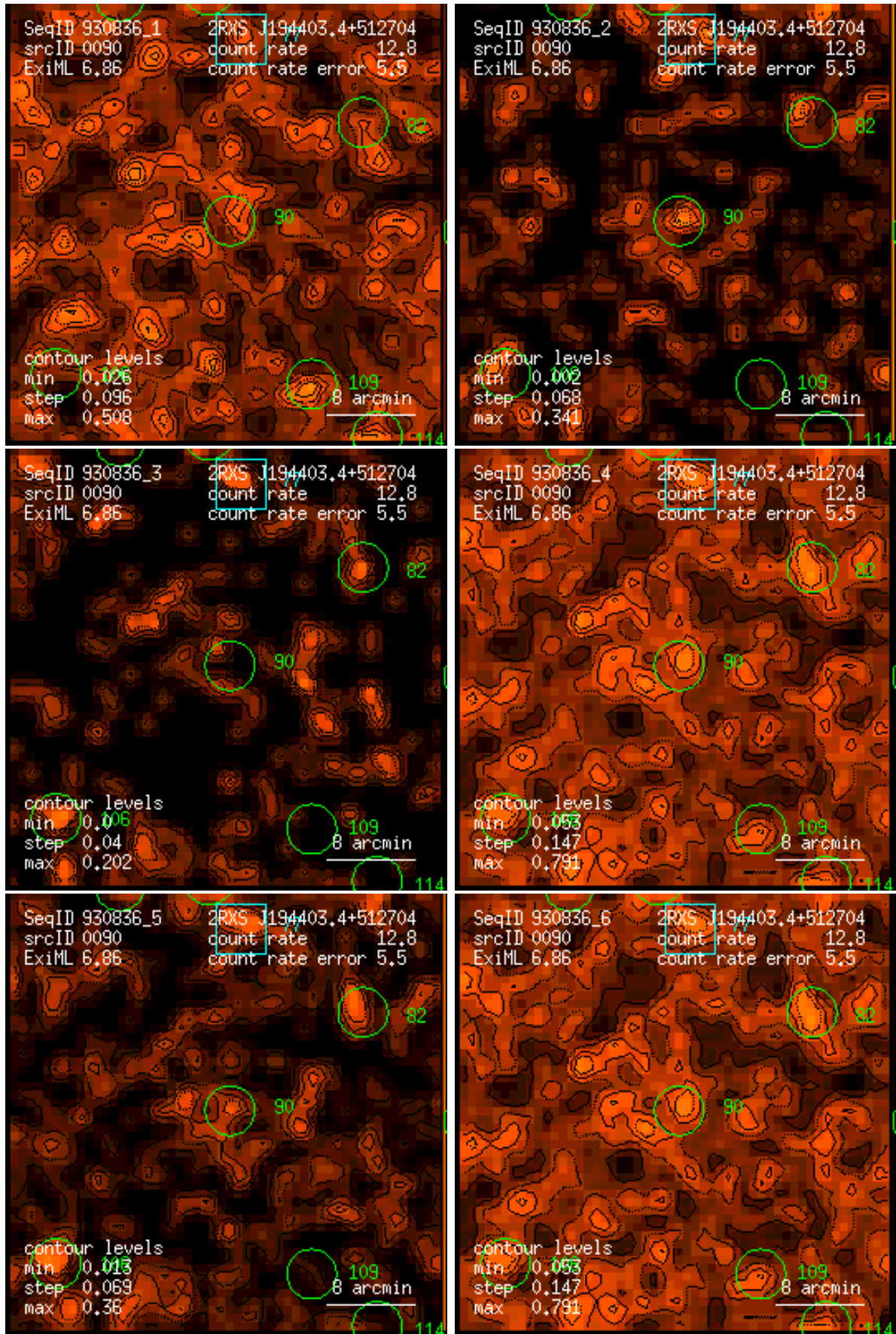
Figure 90: RASS 930836: detection 0090: band rate images, Gaussian filter: (1) PSPC channels 11 – 41, (2) 52 – 90, (3) 91 – 201, (4) 11 – 235, (5) 52 – 201, (6) 11 – 201. Broad band rates in counts/ks. Band rate contour levels in counts/ks/arcmin 2 .
