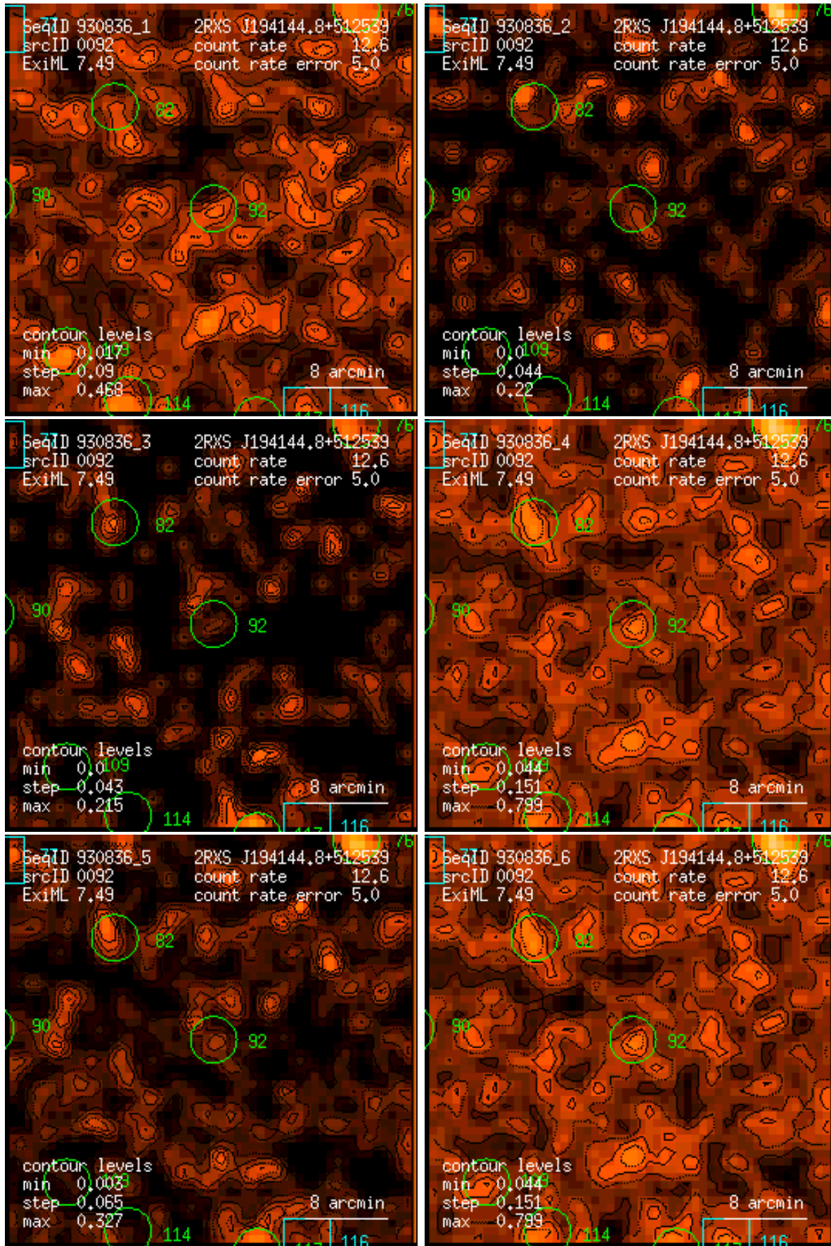
Figure 92: RASS 930836: detection 0092: band rate images, Gaussian filter: (1) PSPC channels 11 – 41, (2) 52 – 90, (3) 91 – 201, (4) 11 – 235, (5) 52 – 201, (6) 11 – 201. Broad band rates in counts/ks. Band rate contour levels in counts/ks/arcmin 2 .
