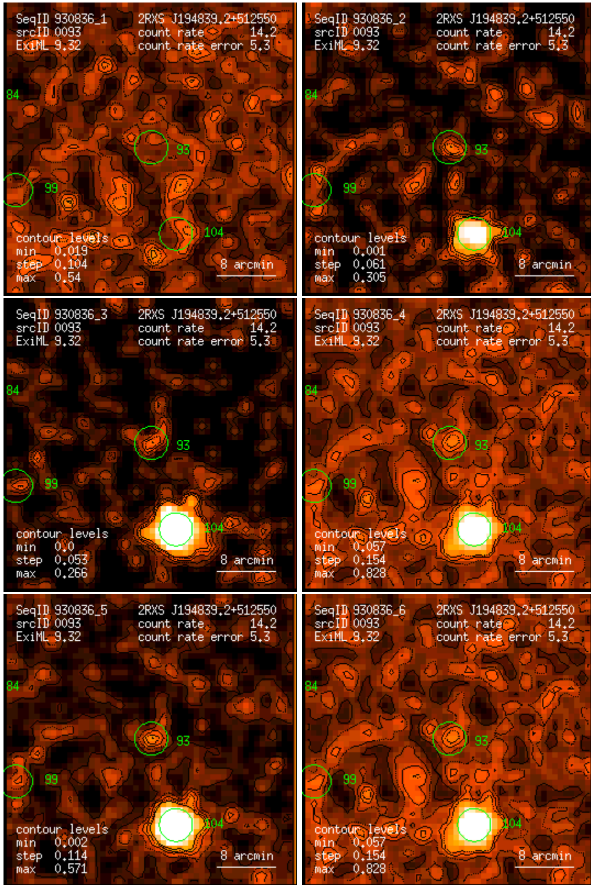
Figure 93: RASS 930836: detection 0093: band rate images, Gaussian filter: (1) PSPC channels 11 – 41, (2) 52 – 90, (3) 91 – 201, (4) 11 – 235, (5) 52 – 201, (6) 11 – 201. Broad band rates in counts/ks. Band rate contour levels in counts/ks/arcmin 2 .
