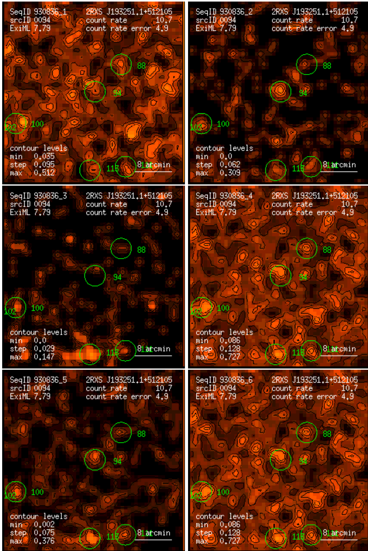
Figure 94: RASS 930836: detection 0094: band rate images, Gaussian filter: (1) PSPC channels 11 – 41, (2) 52 – 90, (3) 91 – 201, (4) 11 – 235, (5) 52 – 201, (6) 11 – 201. Broad band rates in counts/ks. Band rate contour levels in counts/ks/arcmin 2 .
