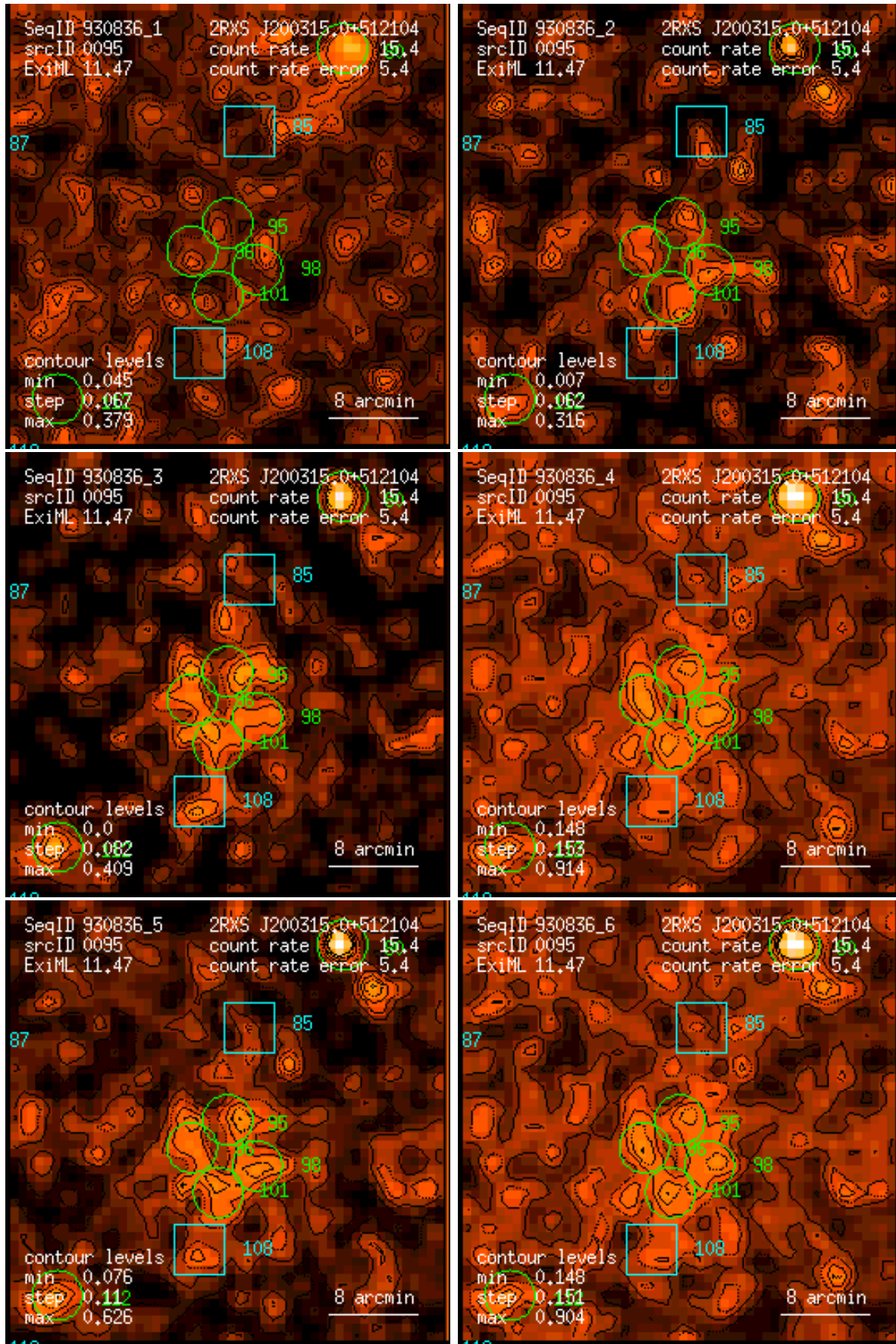
Figure 95: RASS 930836: detection 0095: band rate images, Gaussian filter: (1) PSPC channels 11 – 41, (2) 52 – 90, (3) 91 – 201, (4) 11 – 235, (5) 52 – 201, (6) 11 – 201. Broad band rates in counts/ks. Band rate contour levels in counts/ks/arcmin 2 .
