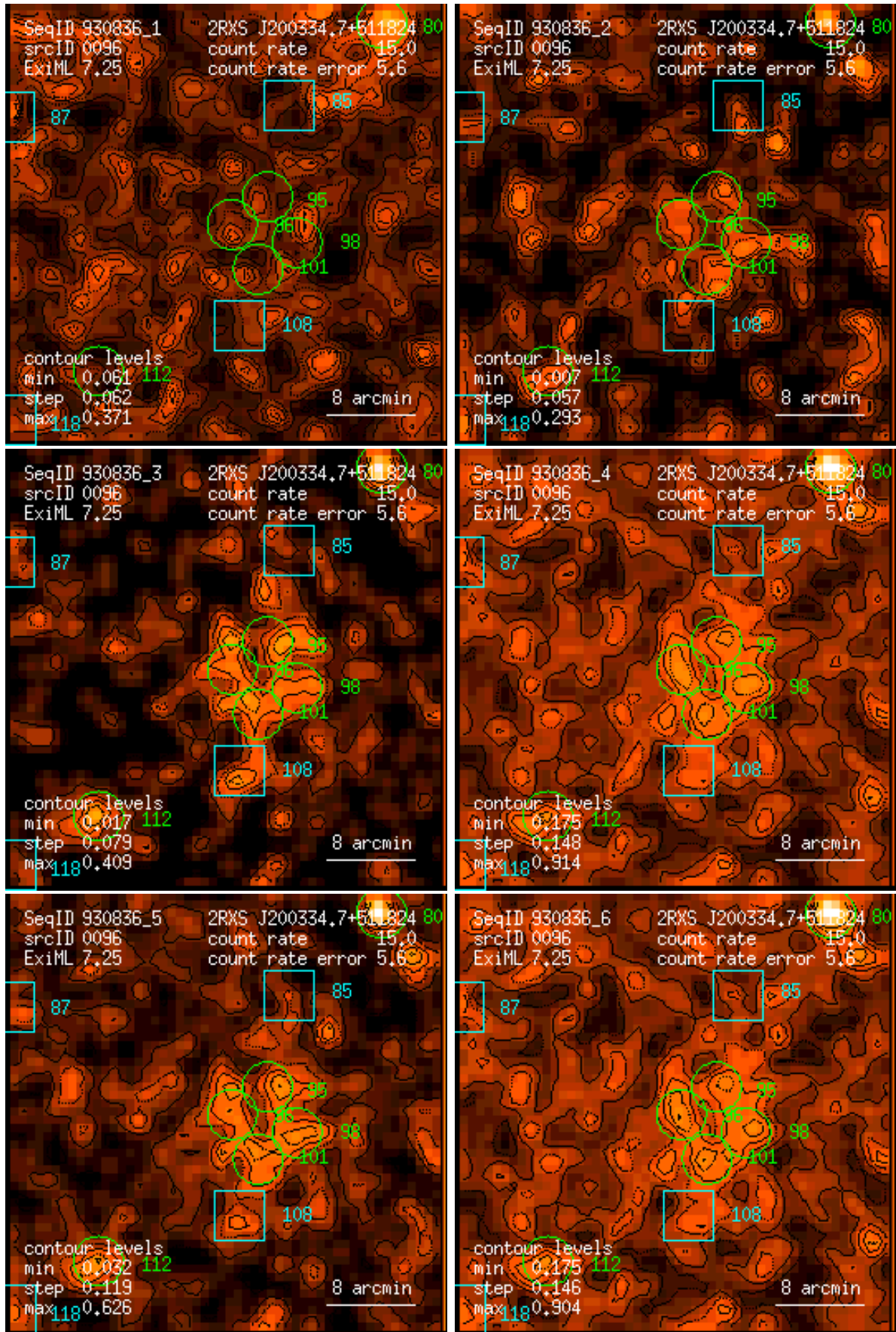
Figure 96: RASS 930836: detection 0096: band rate images, Gaussian filter: (1) PSPC channels 11 – 41, (2) 52 – 90, (3) 91 – 201, (4) 11 – 235, (5) 52 – 201, (6) 11 – 201. Broad band rates in counts/ks. Band rate contour levels in counts/ks/arcmin 2 .
