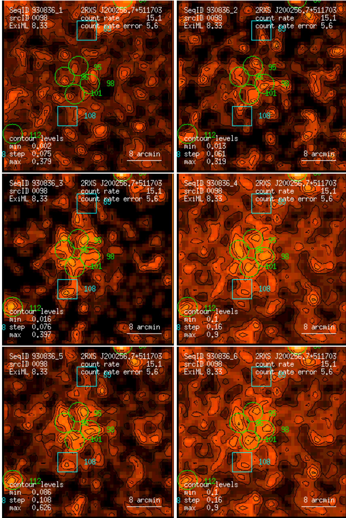
Figure 98: RASS 930836: detection 0098: band rate images, Gaussian filter: (1) PSPC channels 11 – 41, (2) 52 – 90, (3) 91 – 201, (4) 11 – 235, (5) 52 – 201, (6) 11 – 201. Broad band rates in counts/ks. Band rate contour levels in counts/ks/arcmin 2 .
