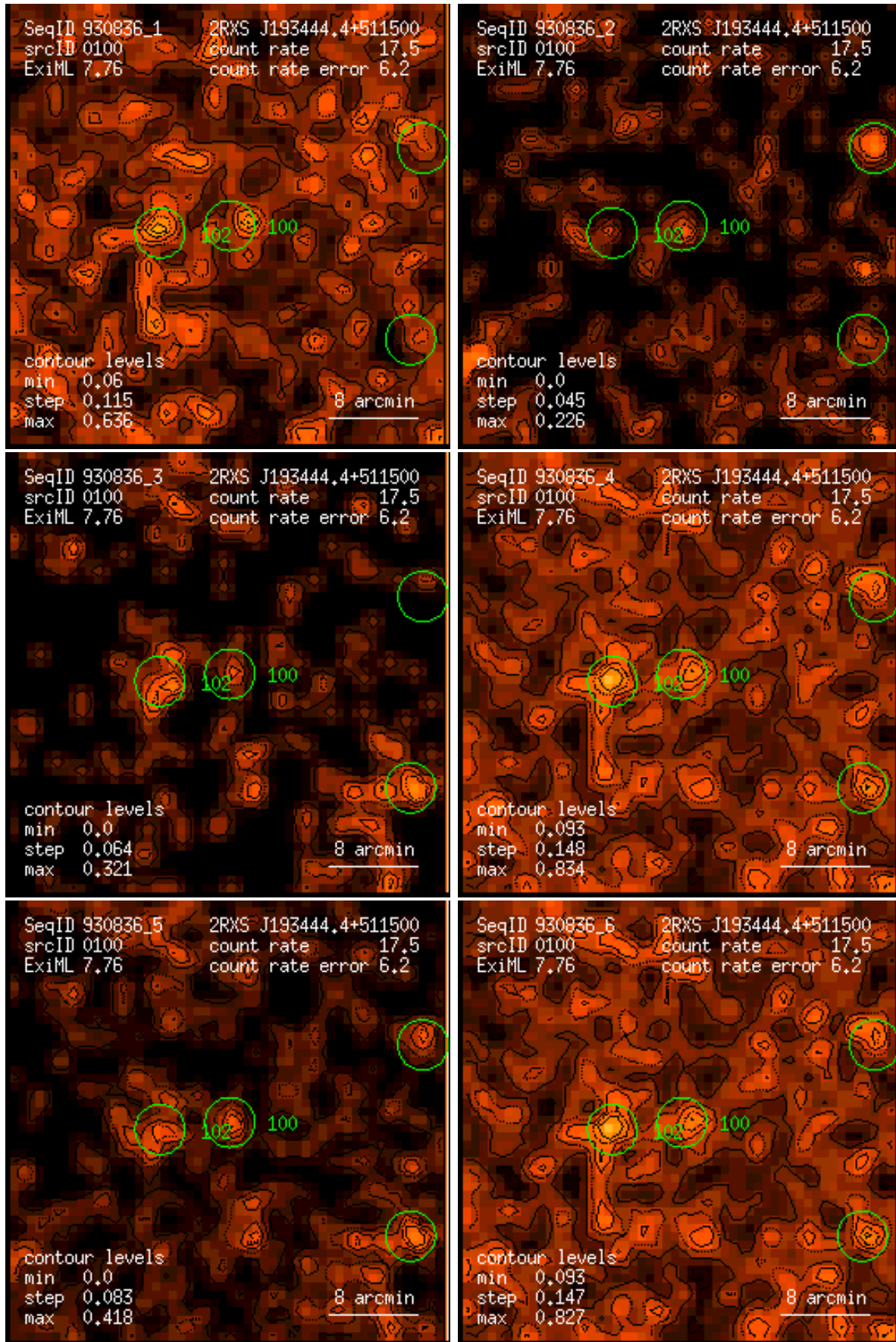
Figure 100: RASS 930836: detection 0100: band rate images, Gaussian filter: (1) PSPC channels 11 – 41, (2) 52 – 90, (3) 91 – 201, (4) 11 – 235, (5) 52 – 201, (6) 11 – 201. Broad band rates in counts/ks. Band rate contour levels in counts/ks/arcmin 2 .
