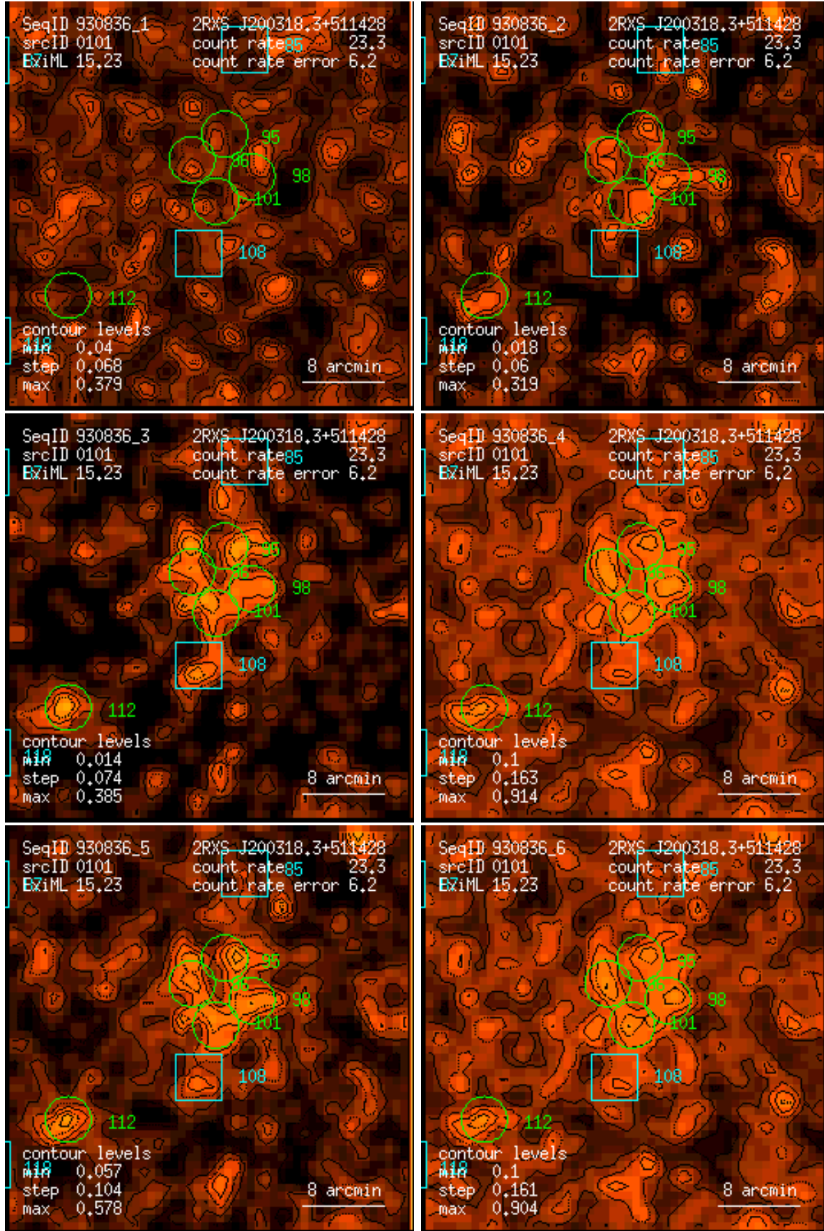
Figure 101: RASS 930836: detection 0101: band rate images, Gaussian filter: (1) PSPC channels 11 – 41, (2) 52 – 90, (3) 91 – 201, (4) 11 – 235, (5) 52 – 201, (6) 11 – 201. Broad band rates in counts/ks. Band rate contour levels in counts/ks/arcmin 2 .
