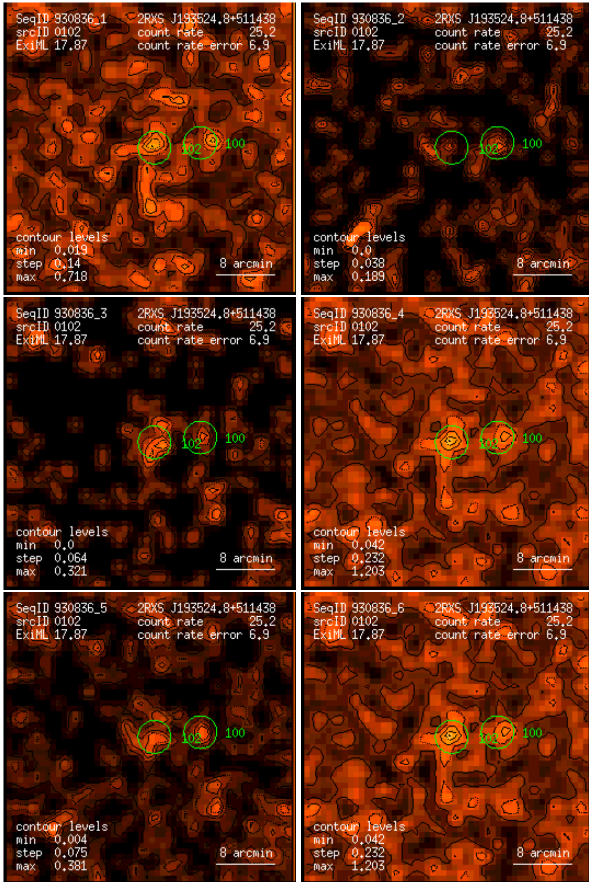
Figure 102: RASS 930836: detection 0102: band rate images, Gaussian filter: (1) PSPC channels 11 – 41, (2) 52 – 90, (3) 91 – 201, (4) 11 – 235, (5) 52 – 201, (6) 11 – 201. Broad band rates in counts/ks. Band rate contour levels in counts/ks/arcmin 2 .
