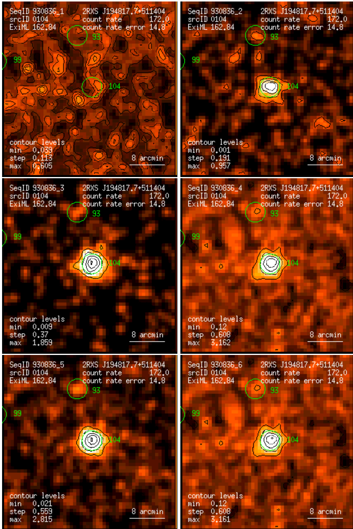
Figure 104: RASS 930836: detection 0104: band rate images, Gaussian filter: (1) PSPC channels 11 – 41, (2) 52 – 90, (3) 91 – 201, (4) 11 – 235, (5) 52 – 201, (6) 11 – 201. Broad band rates in counts/ks. Band rate contour levels in counts/ks/arcmin 2 .
