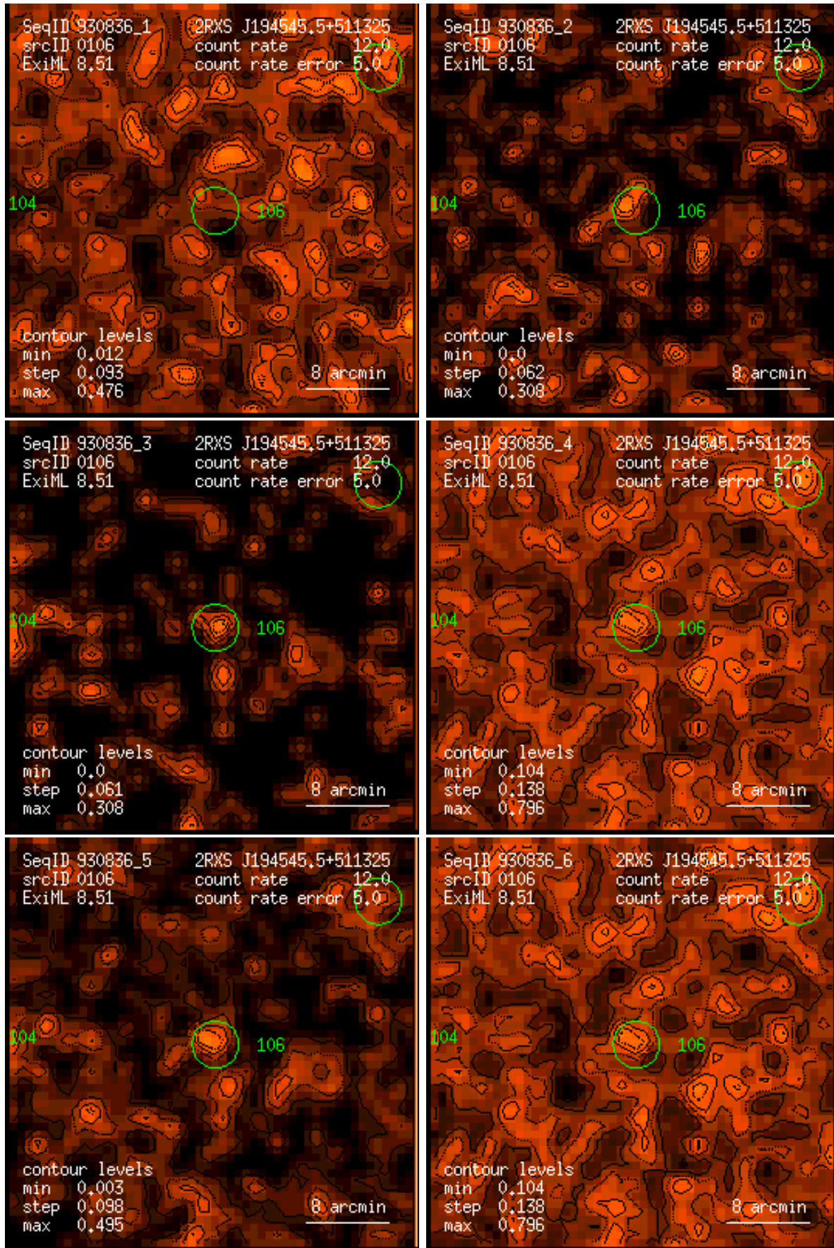
Figure 106: RASS 930836: detection 0106: band rate images, Gaussian filter: (1) PSPC channels 11 – 41, (2) 52 – 90, (3) 91 – 201, (4) 11 – 235, (5) 52 – 201, (6) 11 – 201. Broad band rates in counts/ks. Band rate contour levels in counts/ks/arcmin 2 .
