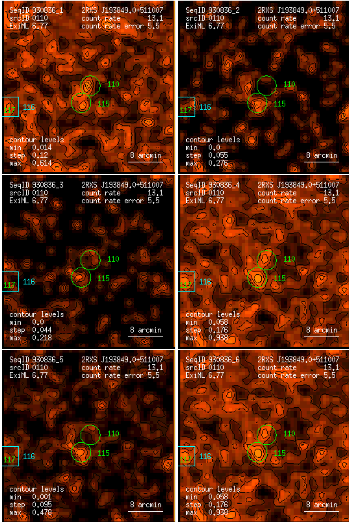
Figure 110: RASS 930836: detection 0110: band rate images, Gaussian filter: (1) PSPC channels 11 – 41, (2) 52 – 90, (3) 91 – 201, (4) 11 – 235, (5) 52 – 201, (6) 11 – 201. Broad band rates in counts/ks. Band rate contour levels in counts/ks/arcmin 2 .
