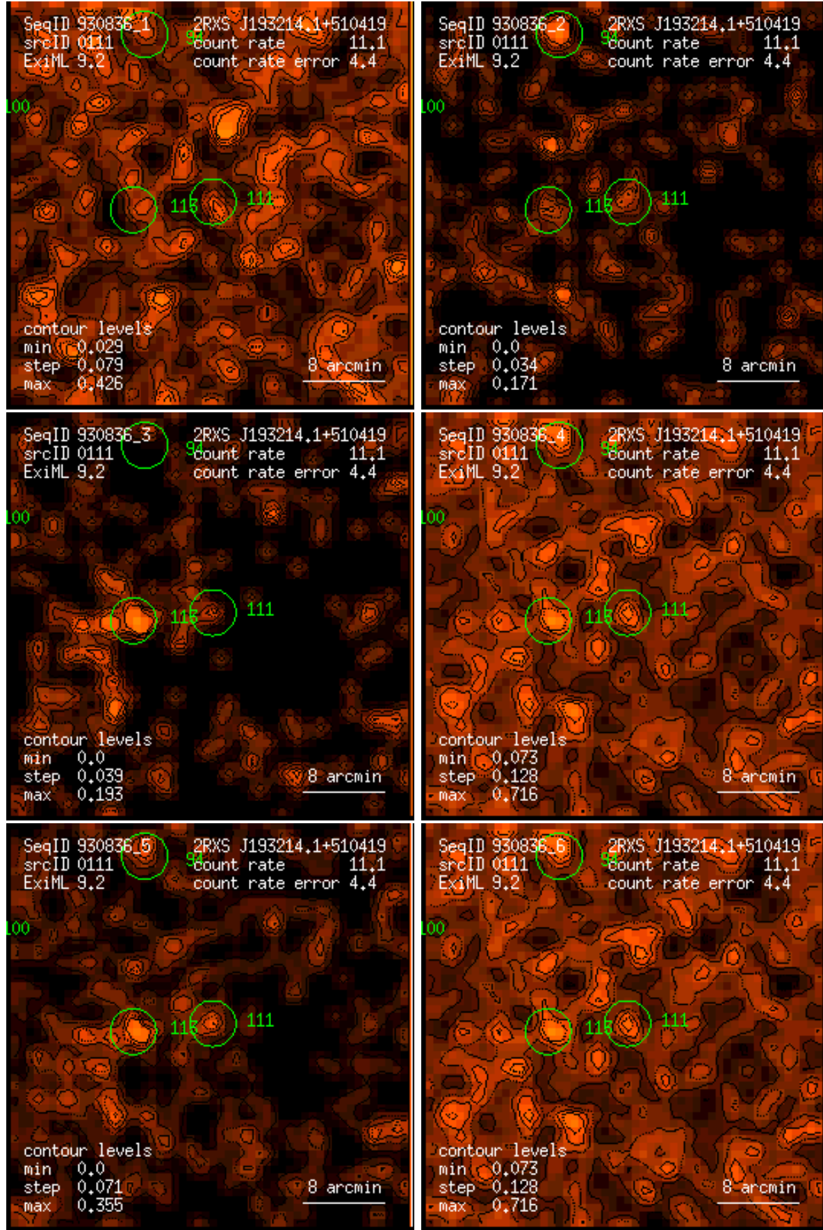
Figure 111: RASS 930836: detection 0111: band rate images, Gaussian filter: (1) PSPC channels 11 – 41, (2) 52 – 90, (3) 91 – 201, (4) 11 – 235, (5) 52 – 201, (6) 11 – 201. Broad band rates in counts/ks. Band rate contour levels in counts/ks/arcmin 2 .
