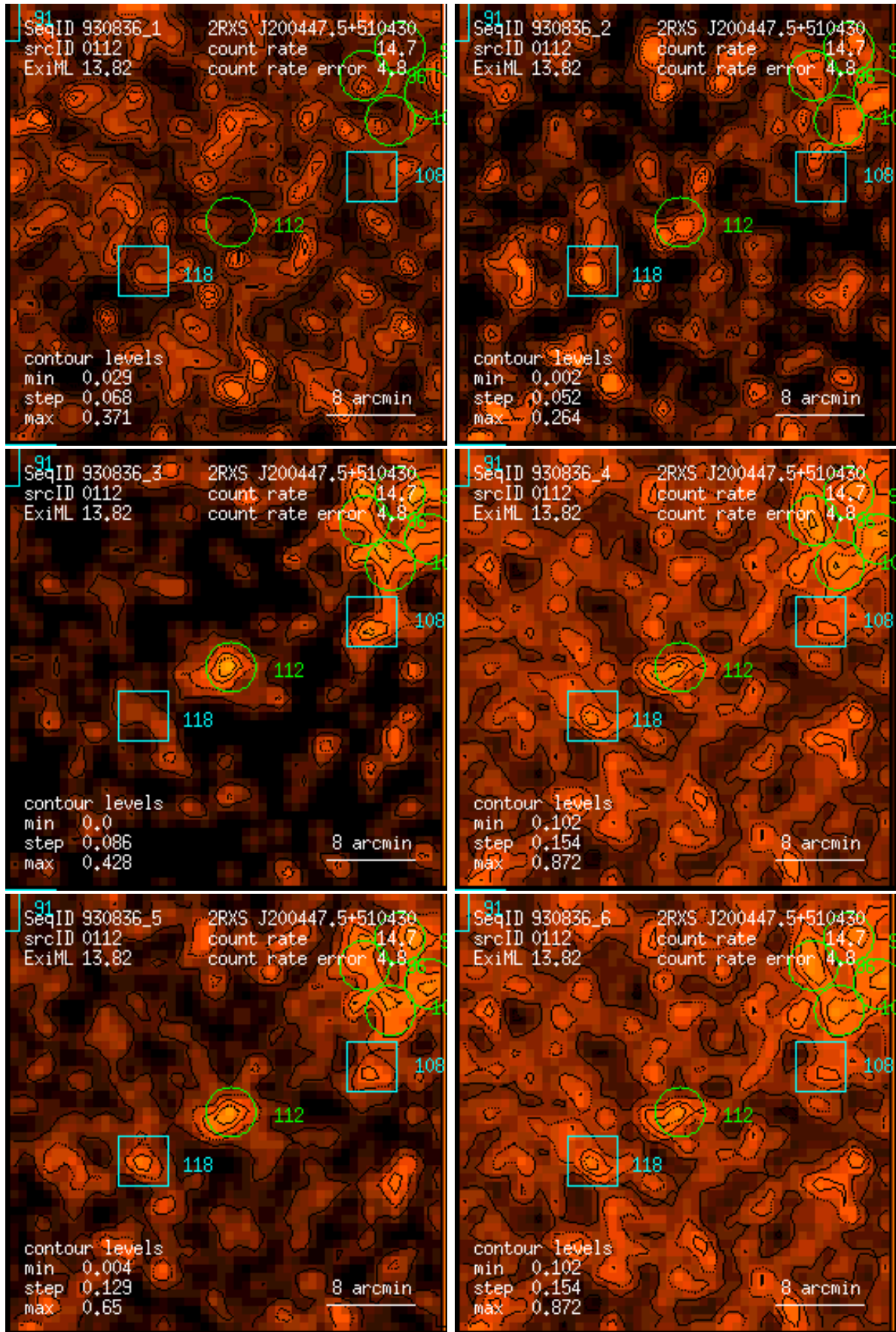
Figure 112: RASS 930836: detection 0112: band rate images, Gaussian filter: (1) PSPC channels 11 – 41, (2) 52 – 90, (3) 91 – 201, (4) 11 – 235, (5) 52 – 201, (6) 11 – 201. Broad band rates in counts/ks. Band rate contour levels in counts/ks/arcmin 2 .
