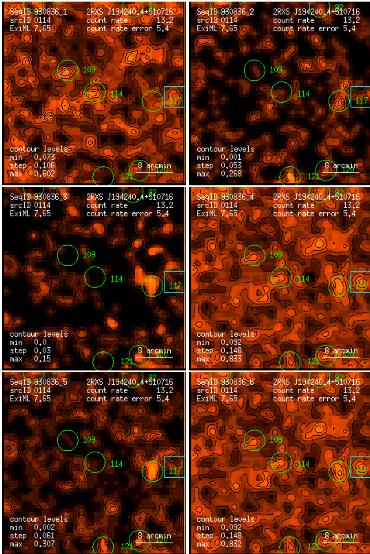
Figure 114: RASS 930836: detection 0114: band rate images, Gaussian filter: (1) PSPC channels 11 – 41, (2) 52 – 90, (3) 91 – 201, (4) 11 – 235, (5) 52 – 201, (6) 11 – 201. Broad band rates in counts/ks. Band rate contour levels in \text{counts/ks/arcmin}^2 .
