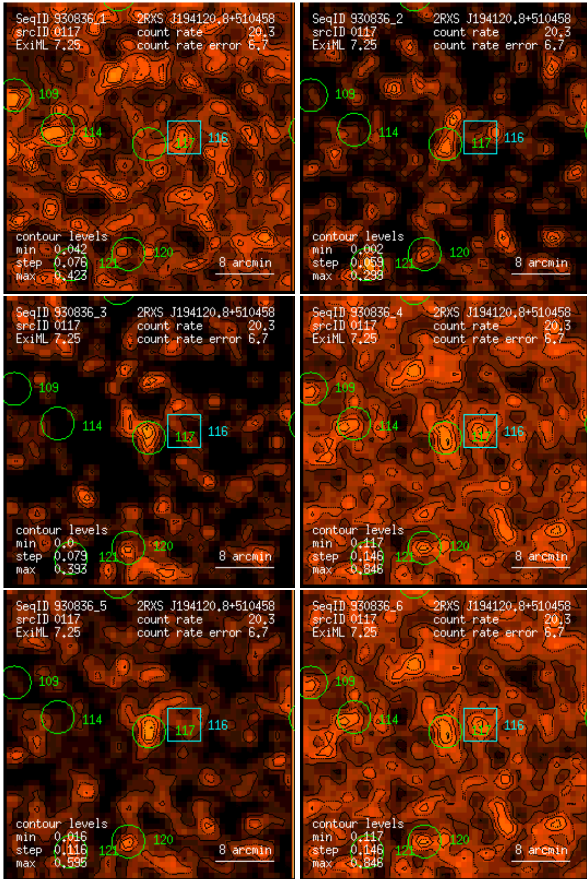
Figure 117: RASS 930836: detection 0117: band rate images, Gaussian filter: (1) PSPC channels 11 – 41, (2) 52 – 90, (3) 91 – 201, (4) 11 – 235, (5) 52 – 201, (6) 11 – 201. Broad band rates in counts/ks. Band rate contour levels in counts/ks/arcmin 2 .
