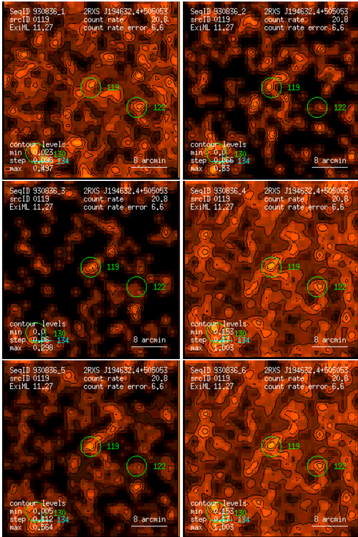
Figure 119: RASS 930836: detection 0119: band rate images, Gaussian filter: (1) PSPC channels 11 – 41, (2) 52 – 90, (3) 91 – 201, (4) 11 – 235, (5) 52 – 201, (6) 11 – 201. Broad band rates in counts/ks. Band rate contour levels in counts/ks/arcmin 2 .
