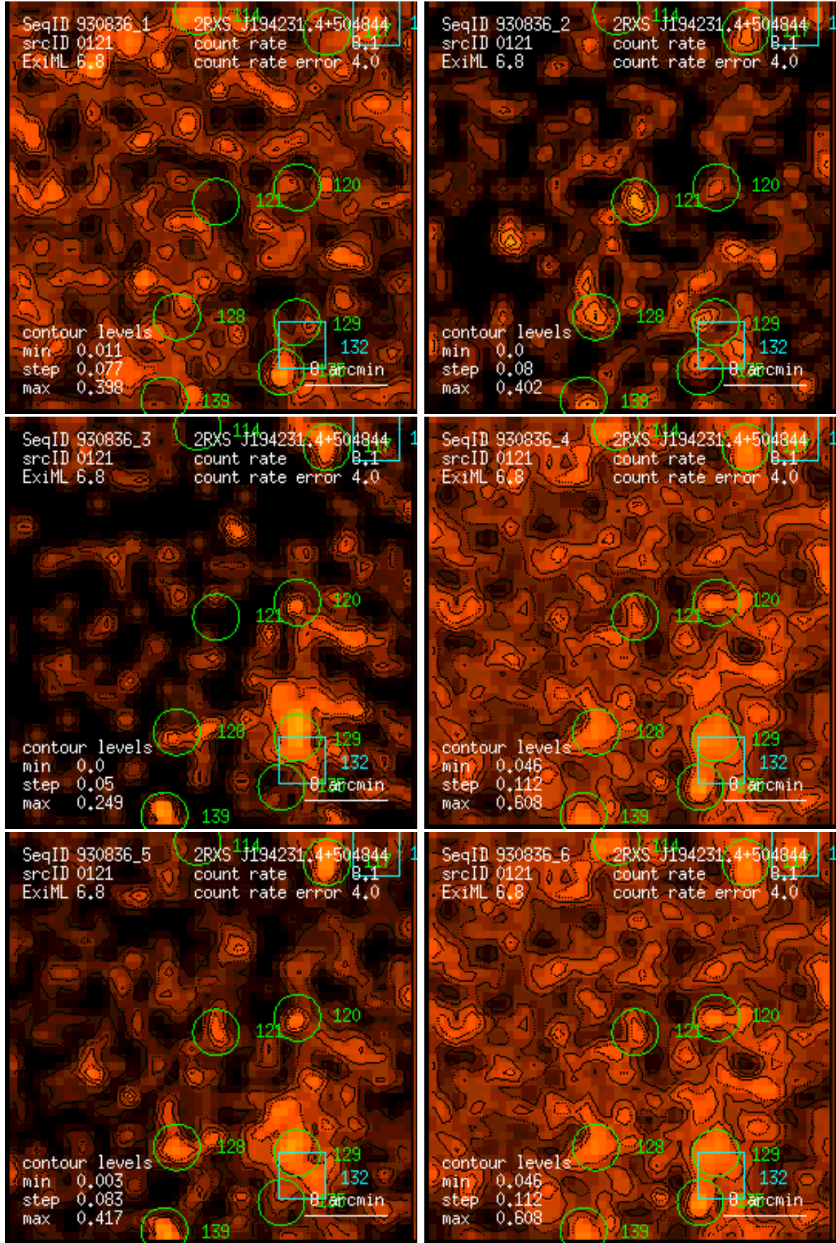
Figure 121: RASS 930836: detection 0121: band rate images, Gaussian filter: (1) PSPC channels 11 – 41, (2) 52 – 90, (3) 91 – 201, (4) 11 – 235, (5) 52 – 201, (6) 11 – 201. Broad band rates in counts/ks. Band rate contour levels in counts/ks/arcmin 2 .
