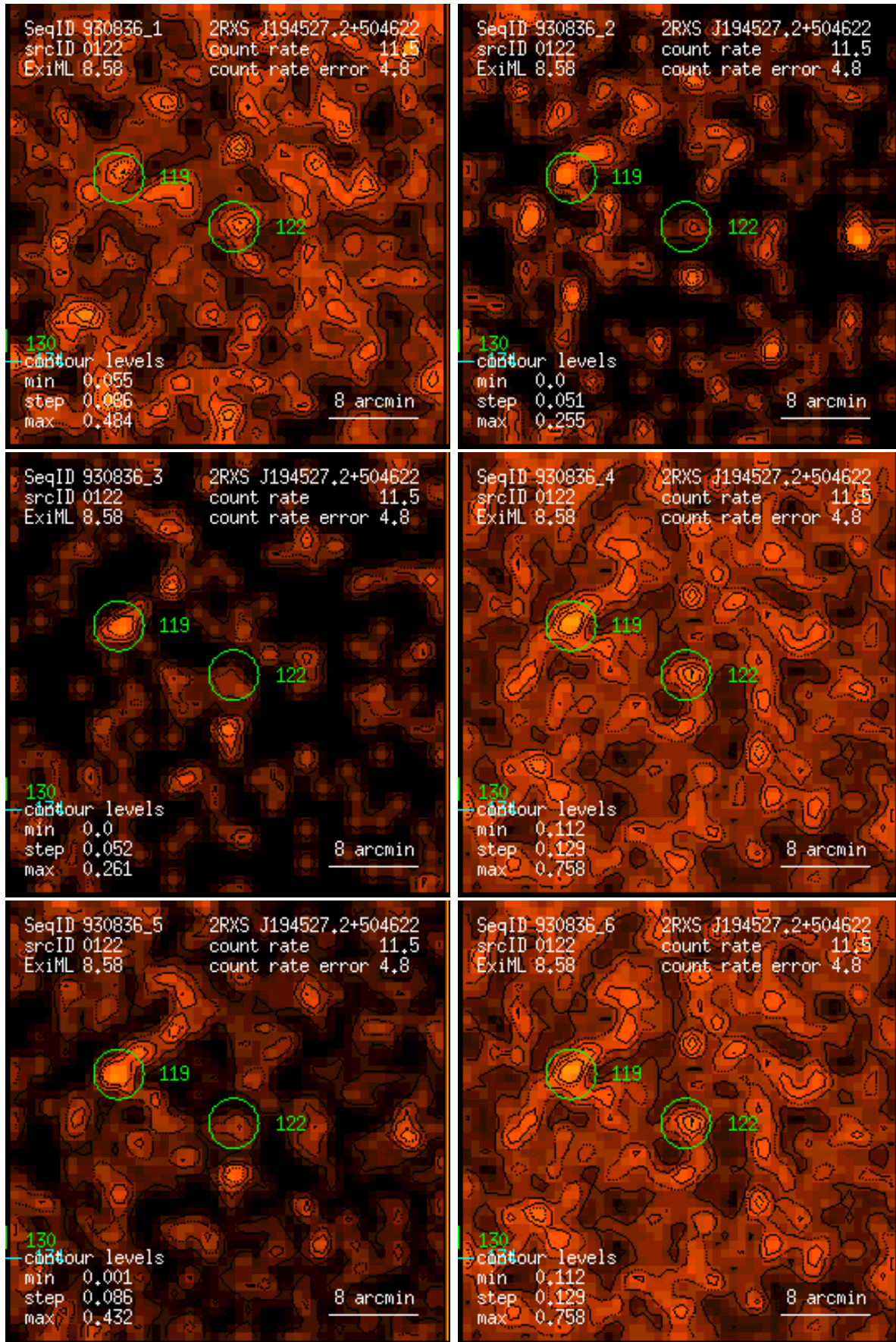
Figure 122: RASS 930836: detection 0122: band rate images, Gaussian filter: (1) PSPC channels 11 – 41, (2) 52 – 90, (3) 91 – 201, (4) 11 – 235, (5) 52 – 201, (6) 11 – 201. Broad band rates in counts/ks. Band rate contour levels in counts/ks/arcmin 2 .
