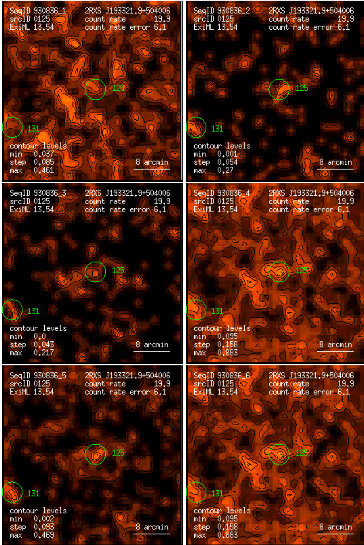
Figure 125: RASS 930836: detection 0125: band rate images, Gaussian filter: (1) PSPC channels 11 – 41, (2) 52 – 90, (3) 91 – 201, (4) 11 – 235, (5) 52 – 201, (6) 11 – 201. Broad band rates in counts/ks. Band rate contour levels in counts/ks/arcmin 2 .
