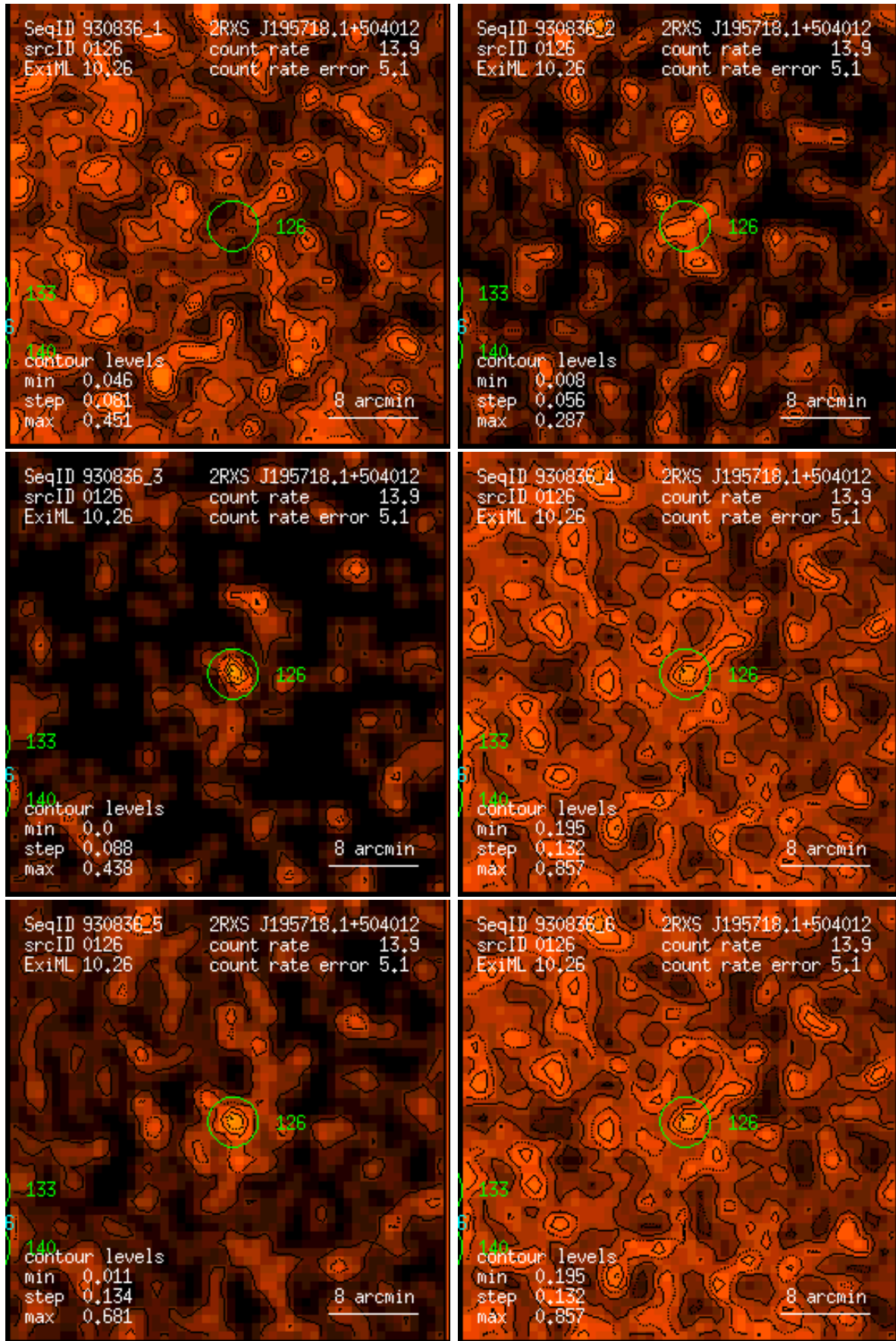
Figure 126: RASS 930836: detection 0126: band rate images, Gaussian filter: (1) PSPC channels 11 – 41, (2) 52 – 90, (3) 91 – 201, (4) 11 – 235, (5) 52 – 201, (6) 11 – 201. Broad band rates in counts/ks. Band rate contour levels in counts/ks/arcmin 2 .
