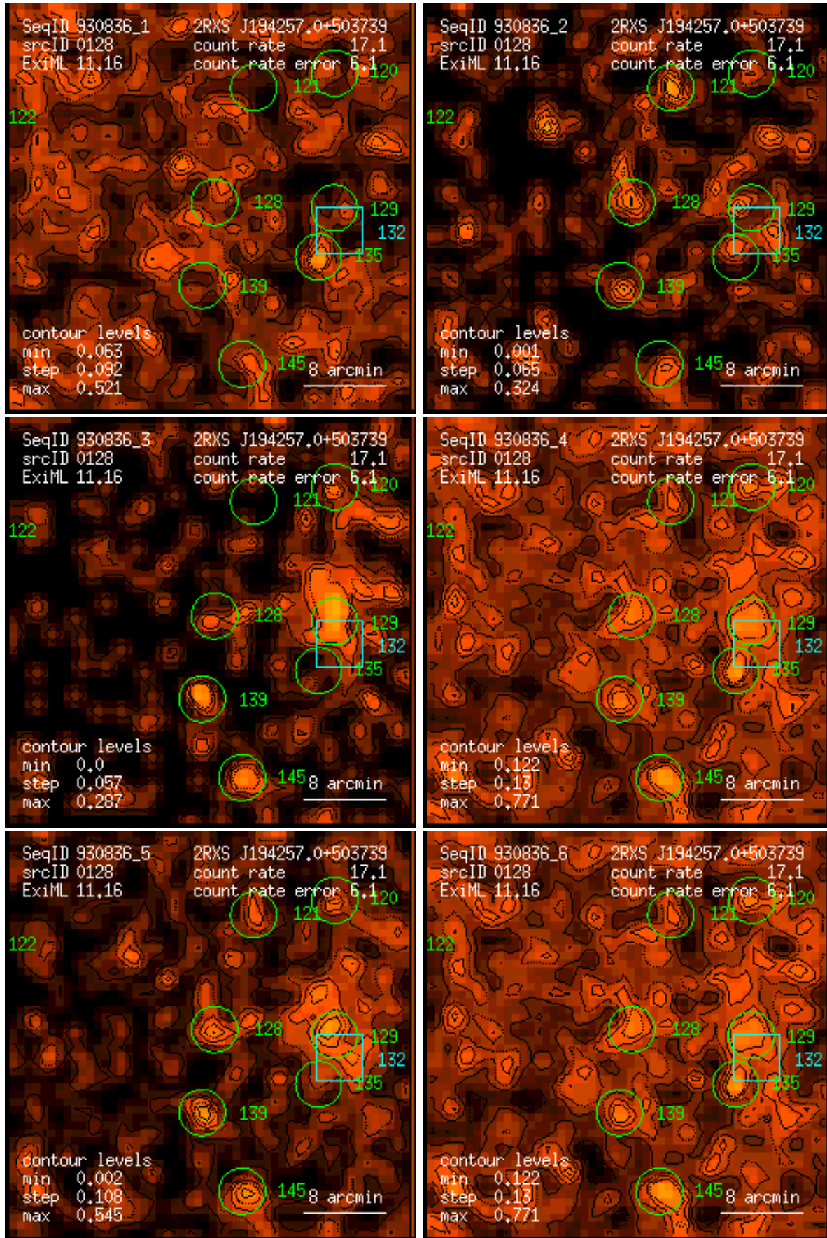
Figure 128: RASS 930836: detection 0128: band rate images, Gaussian filter: (1) PSPC channels 11 – 41, (2) 52 – 90, (3) 91 – 201, (4) 11 – 235, (5) 52 – 201, (6) 11 – 201. Broad band rates in counts/ks. Band rate contour levels in counts/ks/arcmin 2 .
