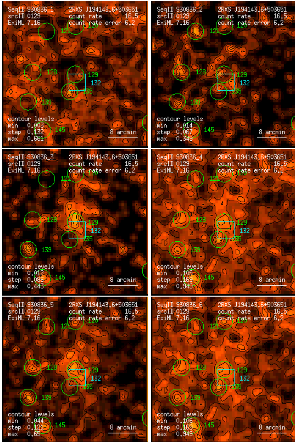
Figure 129: RASS 930836: detection 0129: band rate images, Gaussian filter: (1) PSPC channels 11 – 41, (2) 52 – 90, (3) 91 – 201, (4) 11 – 235, (5) 52 – 201, (6) 11 – 201. Broad band rates in counts/ks. Band rate contour levels in counts/ks/arcmin 2 .
