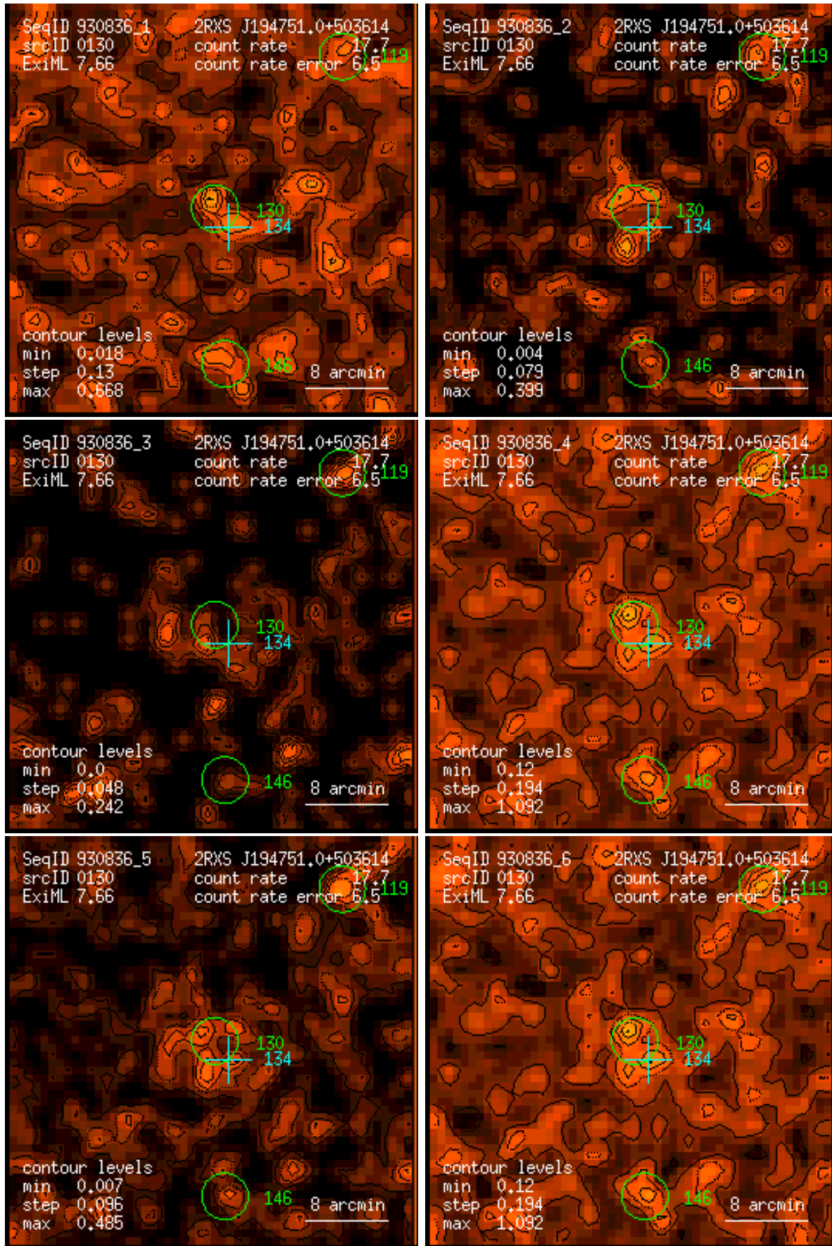
Figure 130: RASS 930836: detection 0130: band rate images, Gaussian filter: (1) PSPC channels 11 – 41, (2) 52 – 90, (3) 91 – 201, (4) 11 – 235, (5) 52 – 201, (6) 11 – 201. Broad band rates in counts/ks. Band rate contour levels in counts/ks/arcmin 2 .
